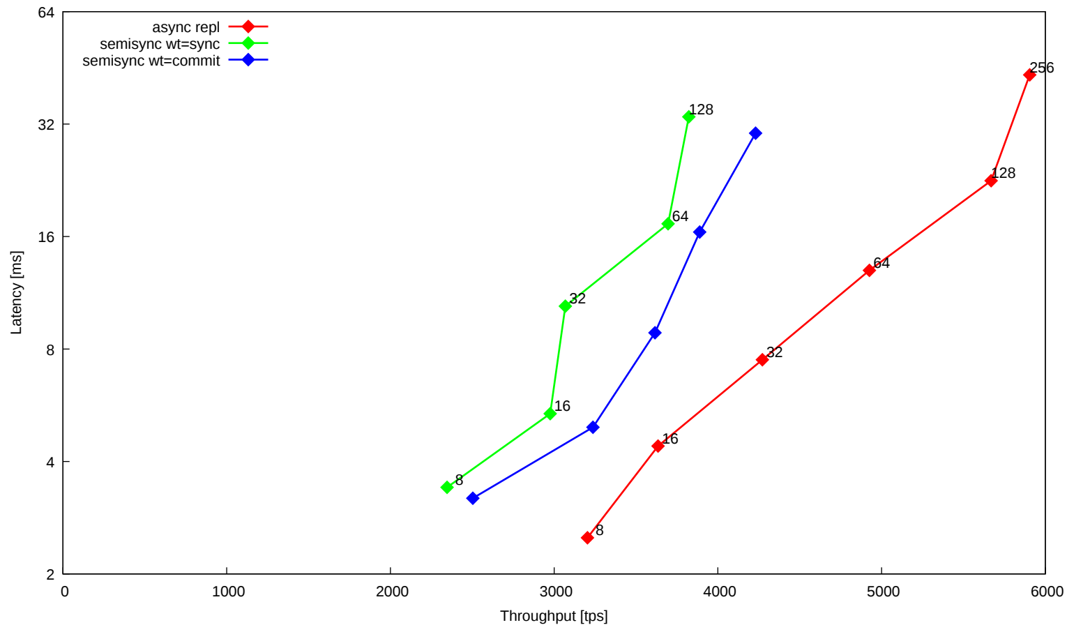
OLTP update indexed (Master only)
