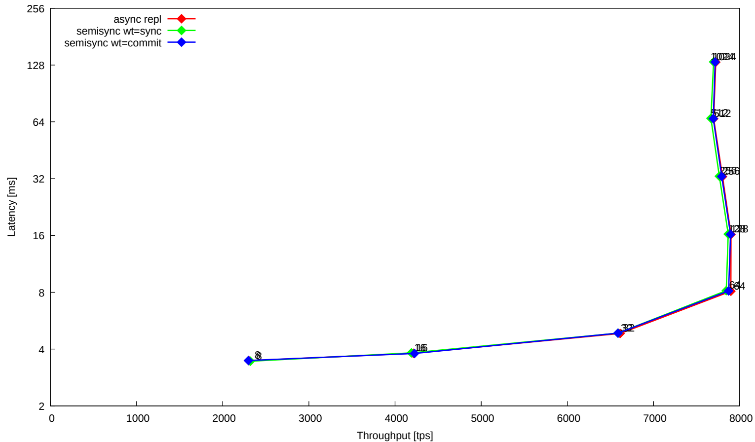
OLTP read/write 10% writes (through MaxScale)
