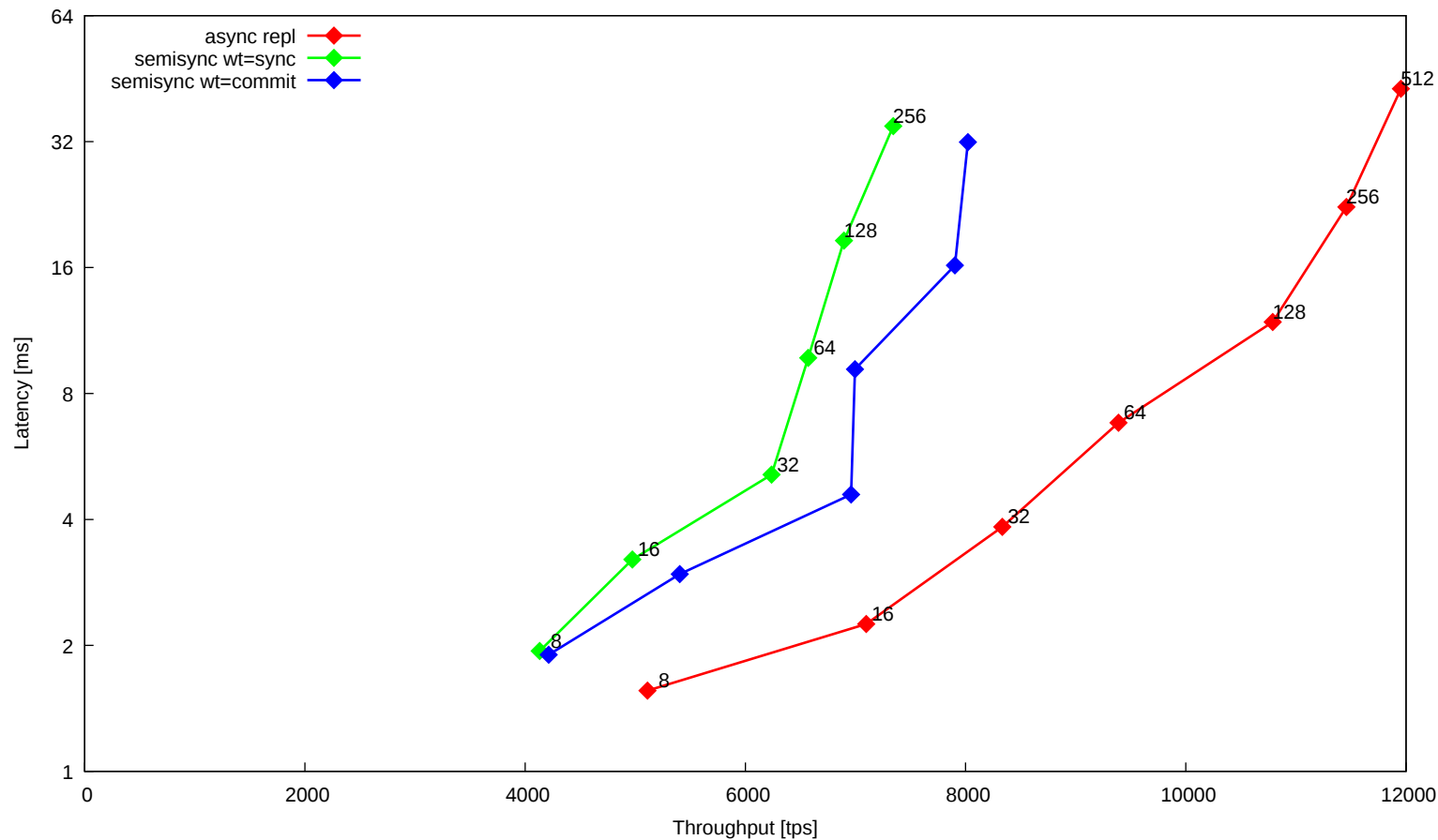
OLTP write-only (Master only)
