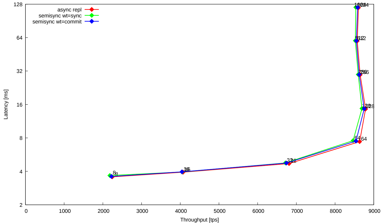
OLTP read/write 25% writes (through MaxScale)
