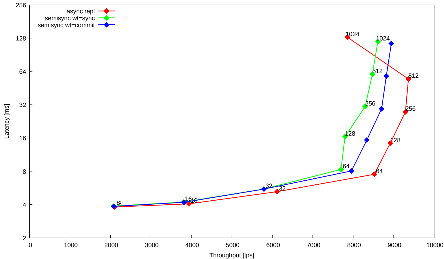
OLTP read/write 50% writes (through MaxScale)
