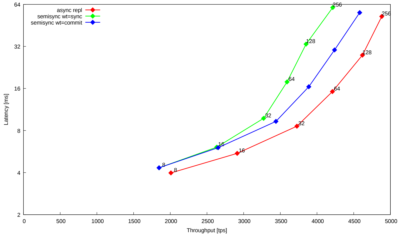
OLTP read/write (Master only)
