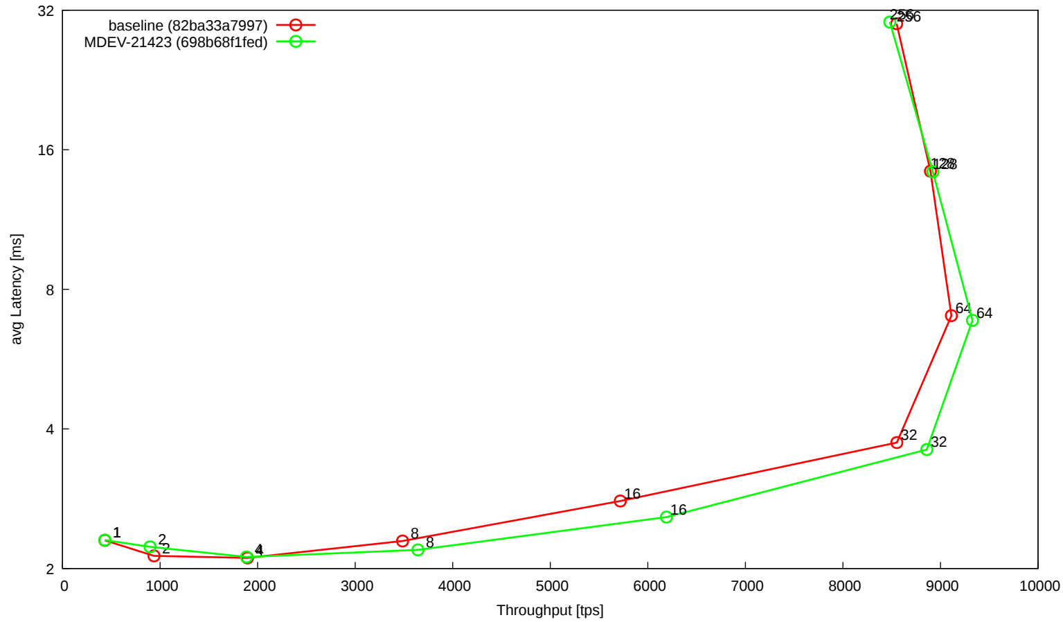
t_oltp_full_innodb (@cheetah02)
