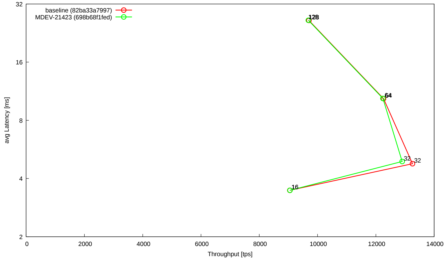
t_tprocc (@cheetah02)
