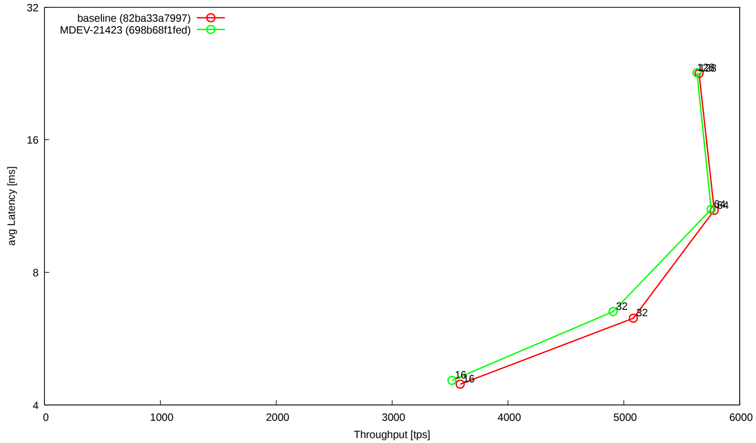
t_sysbench_tpcc (@cheetah02)
