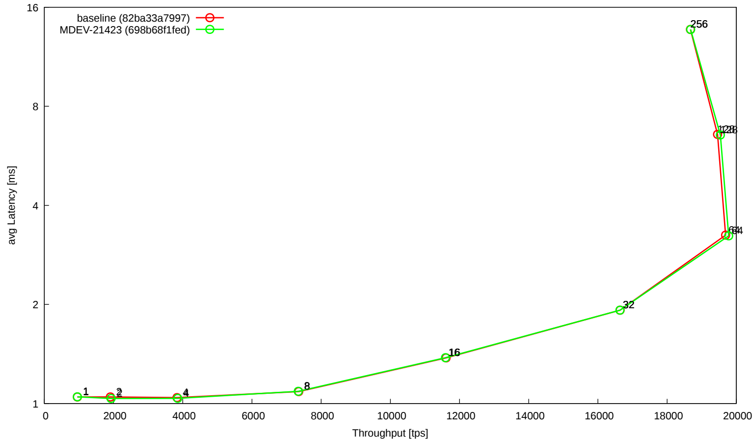
t_oltp_insert_innodb_batched (@cheetah02)
