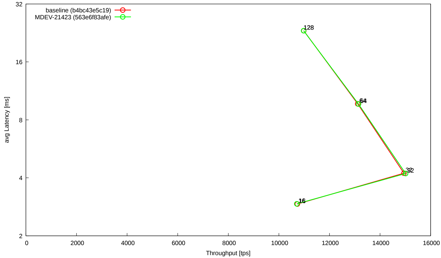
t_tprocc (@cheetah02)
