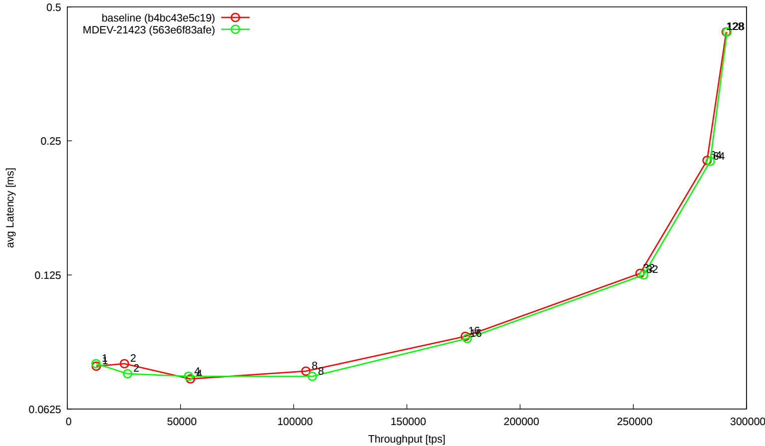
t_oltp_pointselect_innodb (@cheetah02)
