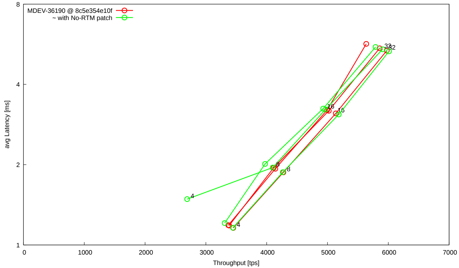
t_oltp_writes_innodb, innodb_read_ahead=on
