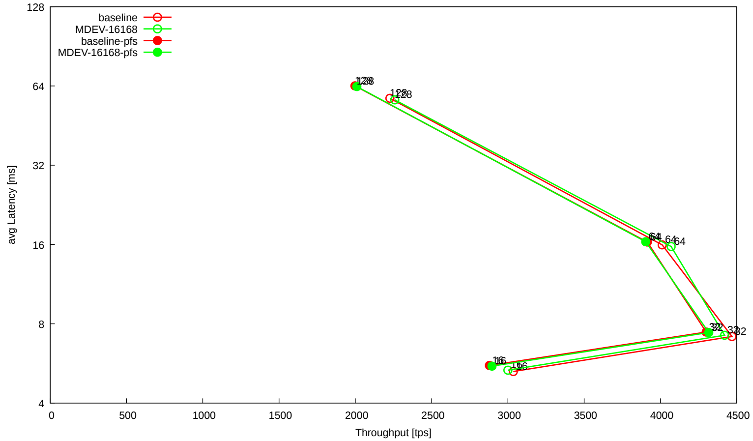
workload 't_sysbench_tpcc_big'
