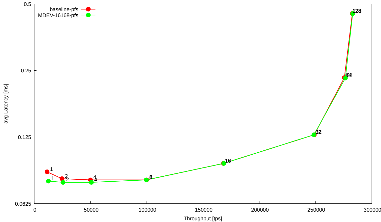
workload 't_oltp_pointselect_innodb'
