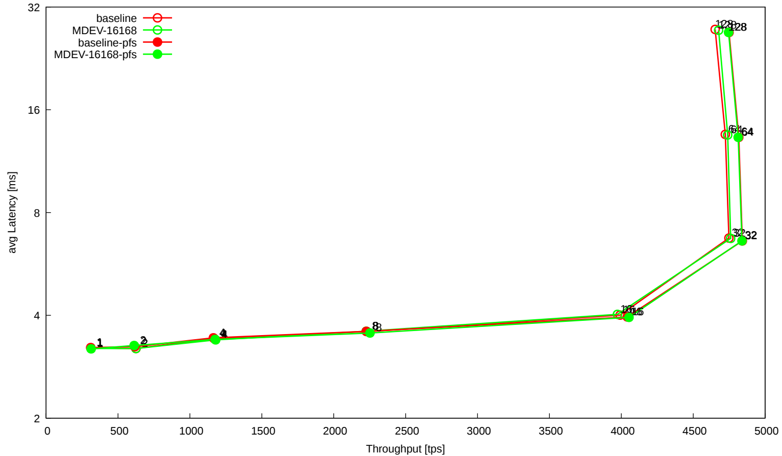
workload 't_oltp_order_big_ranges'
