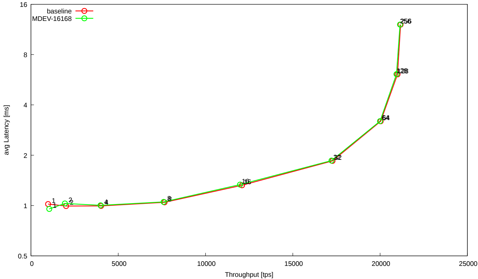
workload 't_oltp_insert_innodb_batched'
