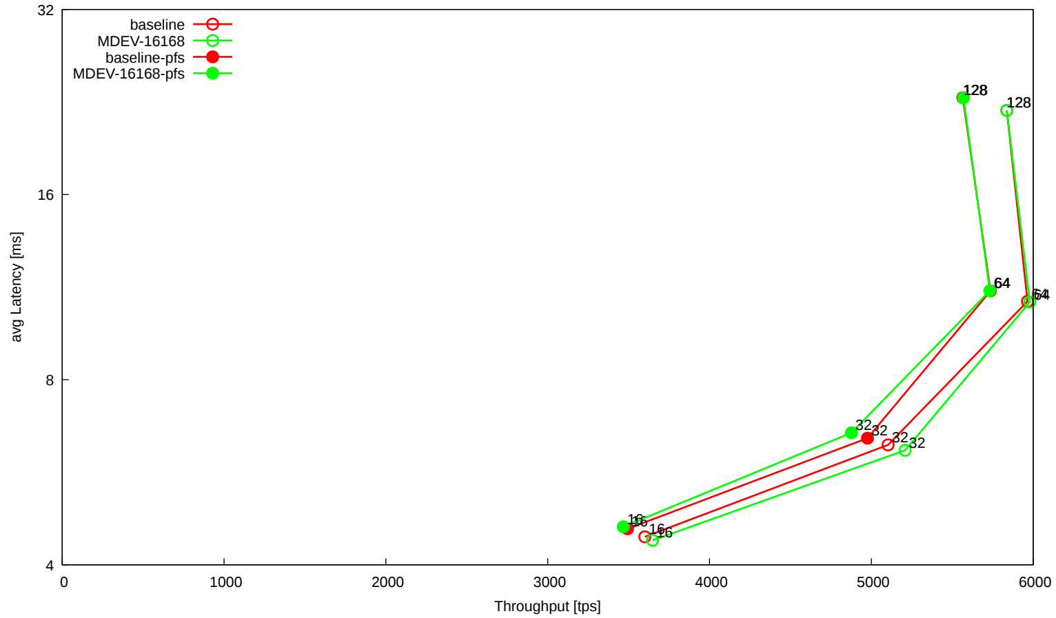
workload 't_sysbench_tpcc'
