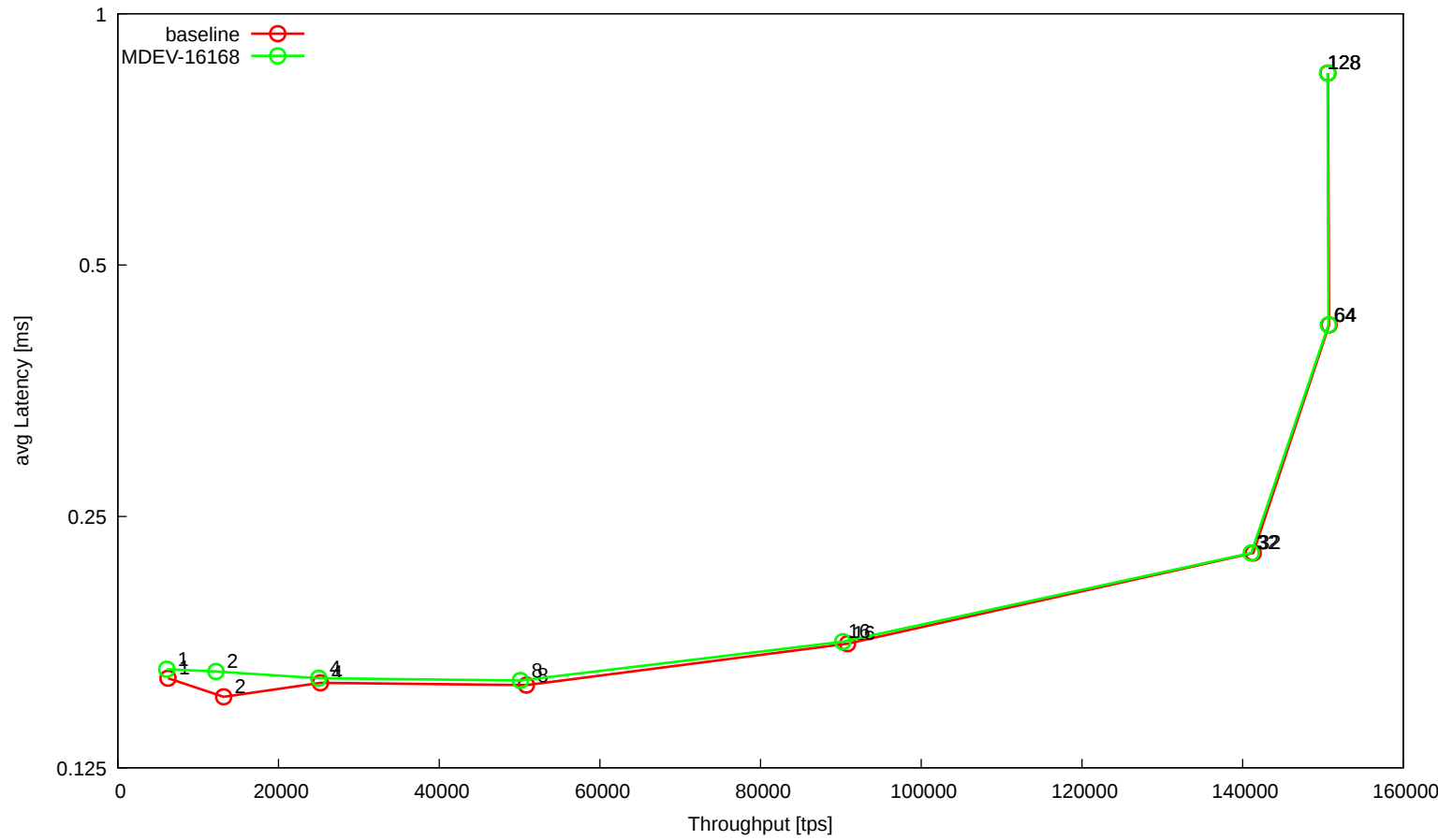
workload 't_collate_utf8_general'
