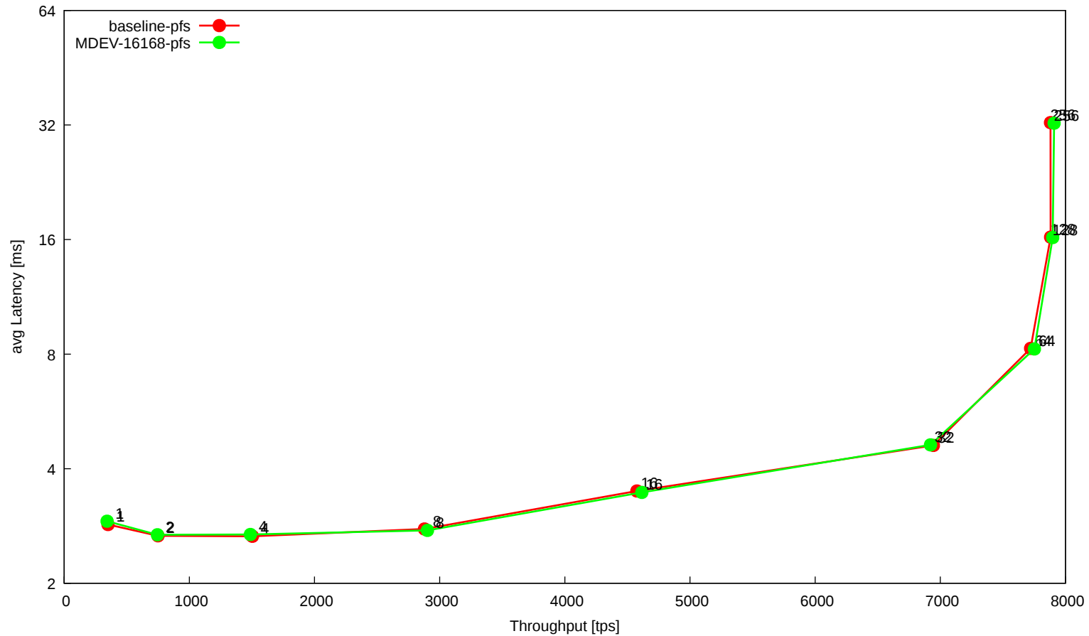
workload 't_oltp_full_innodb'
