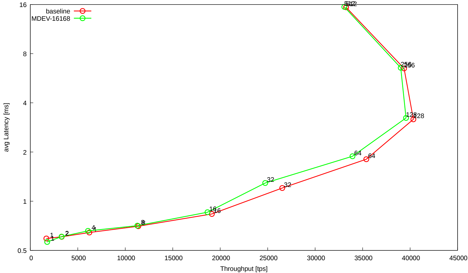
workload 't_oltp_writes_innodb'
