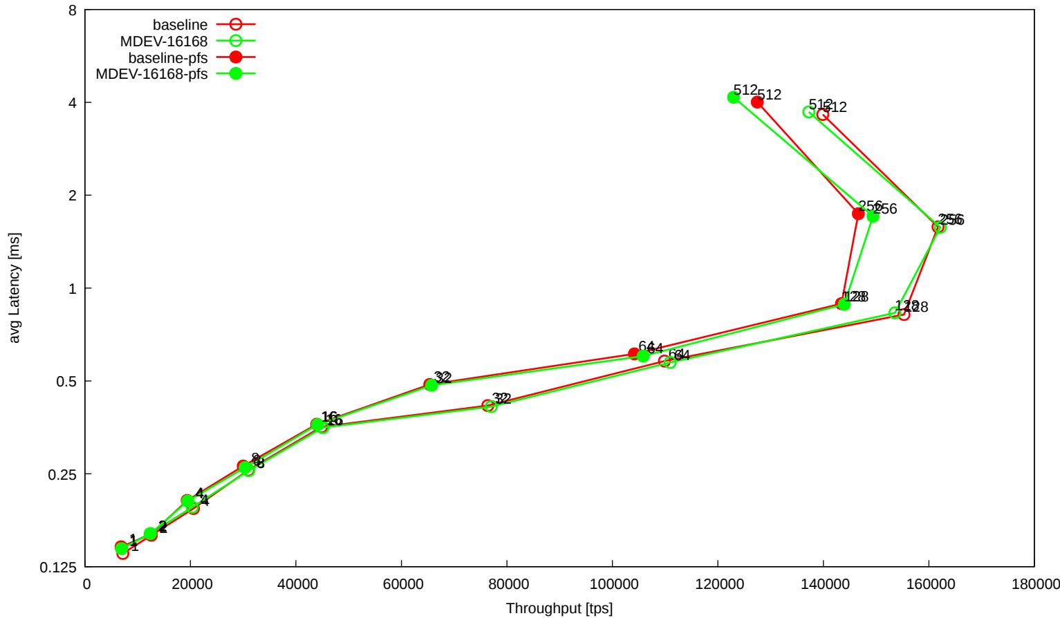
workload 't_otp_insert_innodb'
