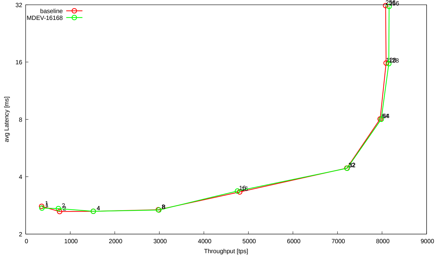
workload 't_oltp_full_innodb'
