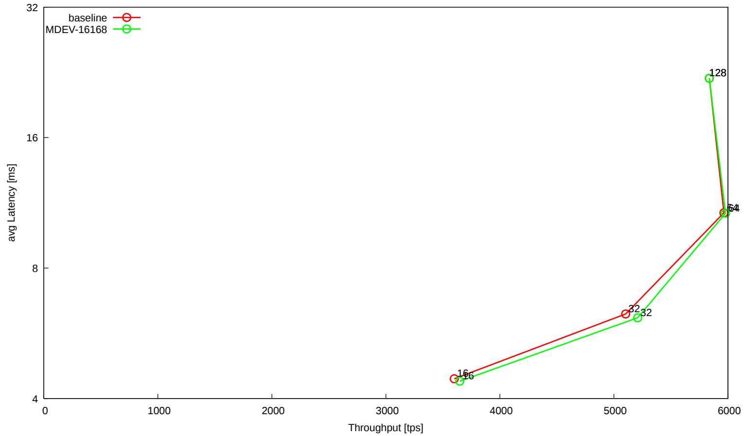
workload 't_sysbench_tpcc'
