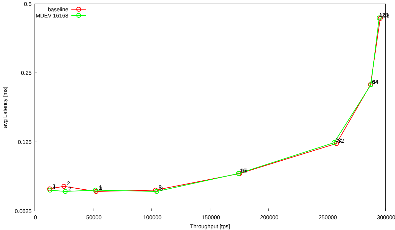
workload 't_oltp_pointselect_innodb'
