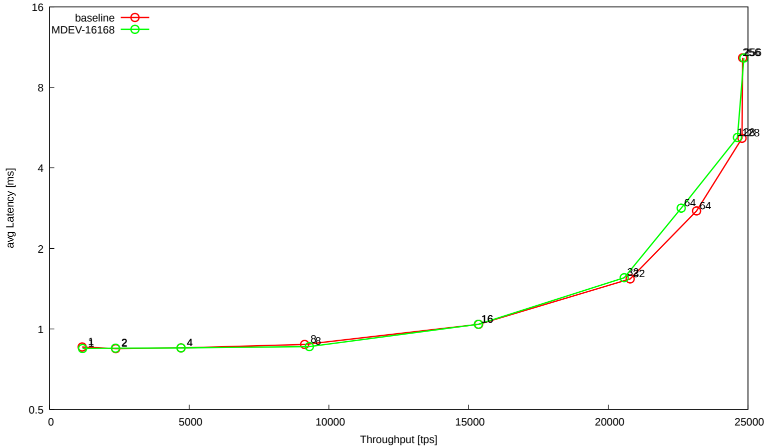
workload 't_oltp_9010_innodb'
