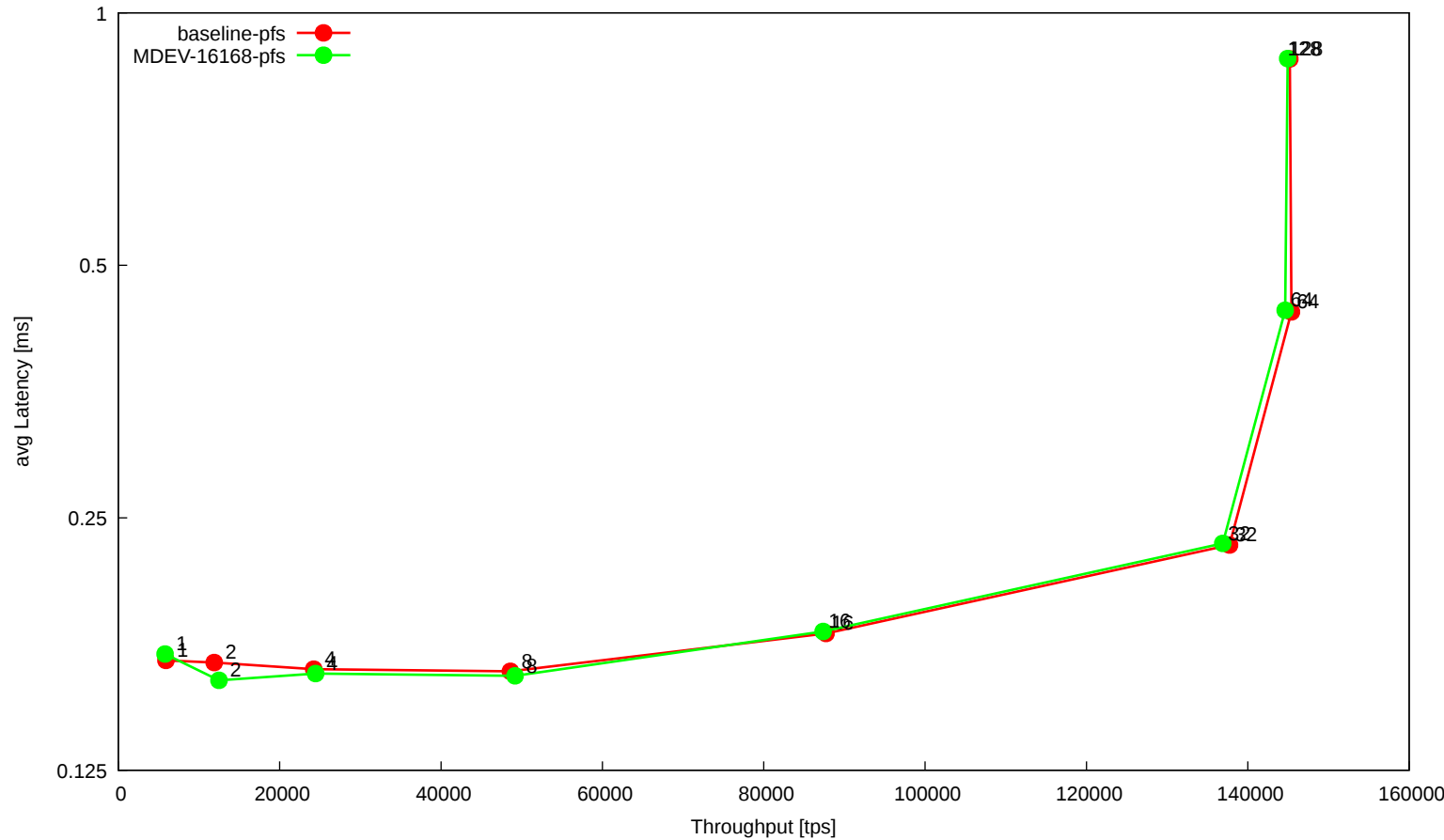
workload 't_collate_utf8_general'
