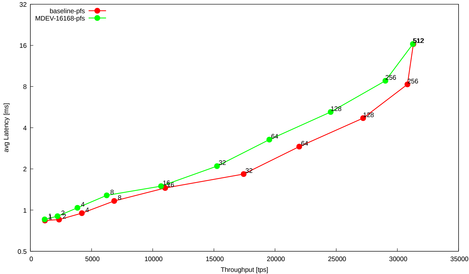
workload 't_oltp_writes_innodb_binlog'
