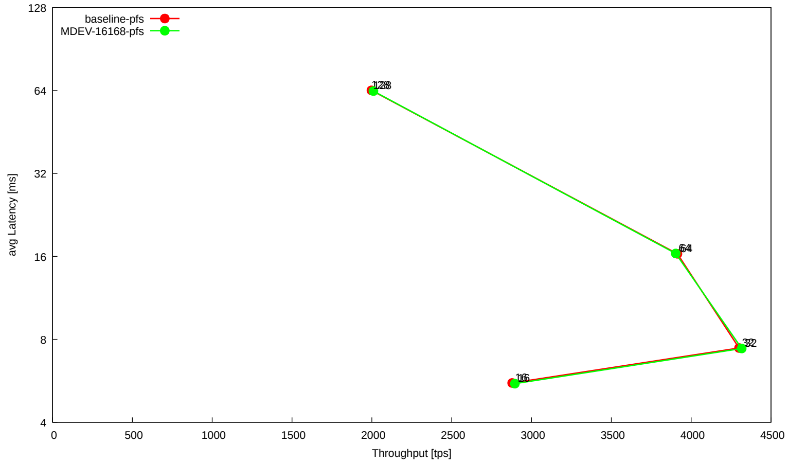
workload 't_sysbench_tpcc_big'
