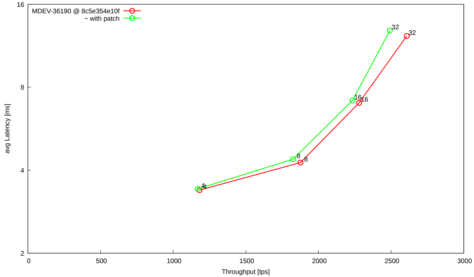
t_sysbench_tpcc_big
