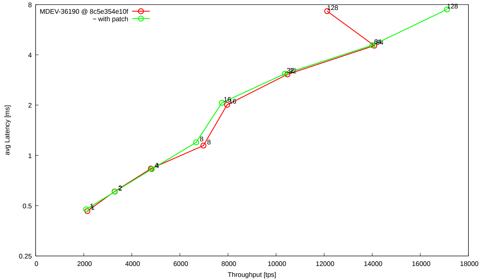
t_oltp_writes_innodb
