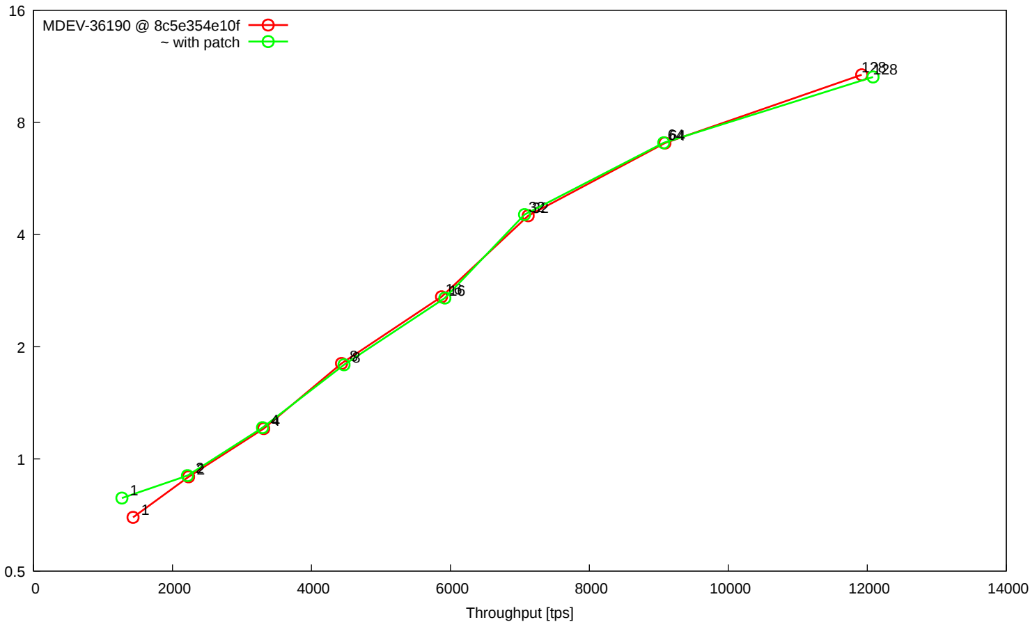
t_oltp_writes_innodb_binlog
