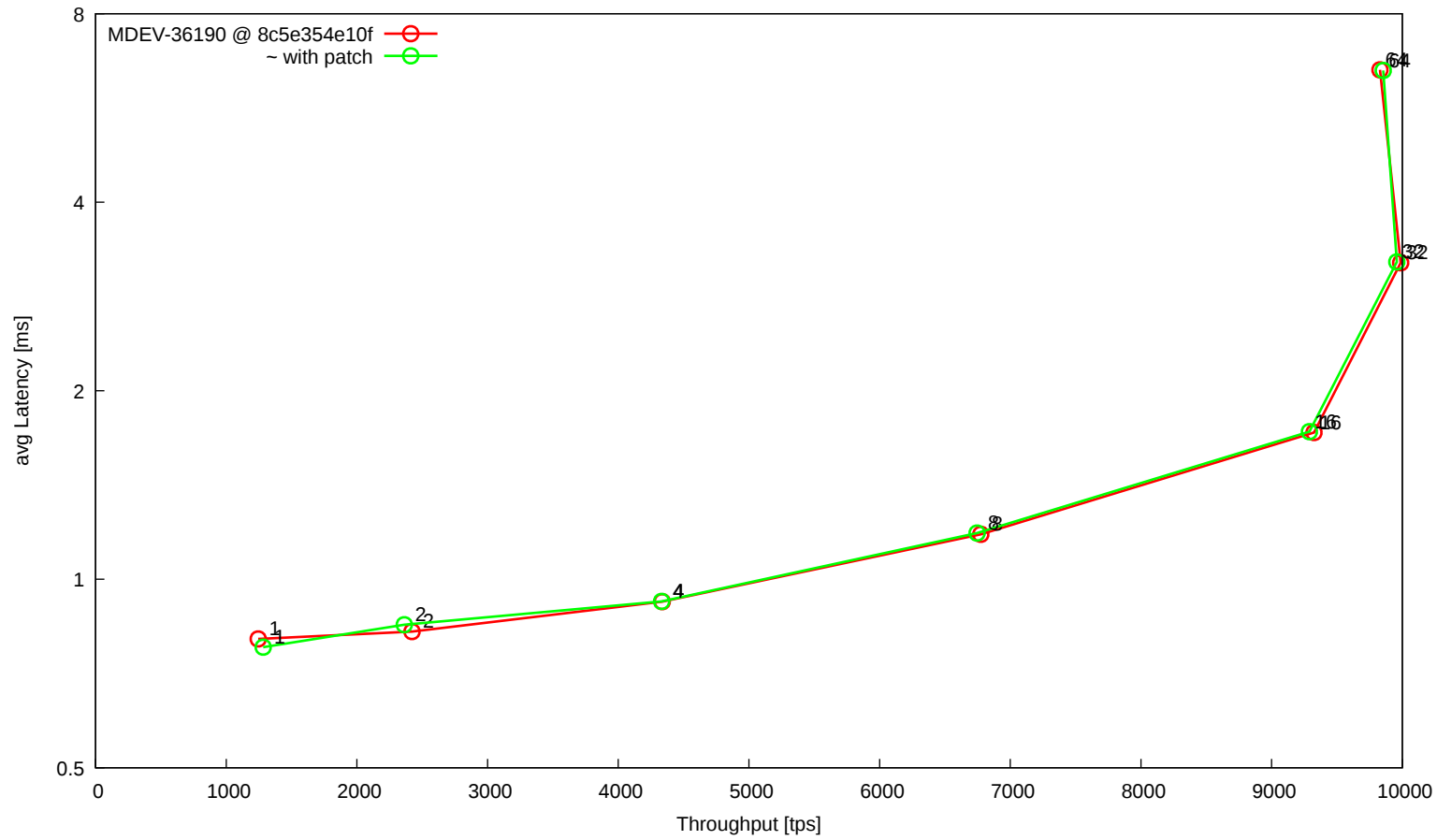
t_oltp_insert_innodb_batched
