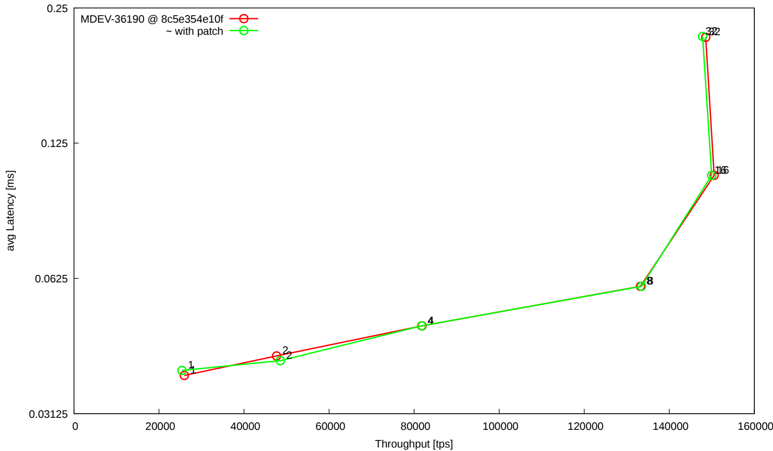
t_oltp_pointselect_innodb
