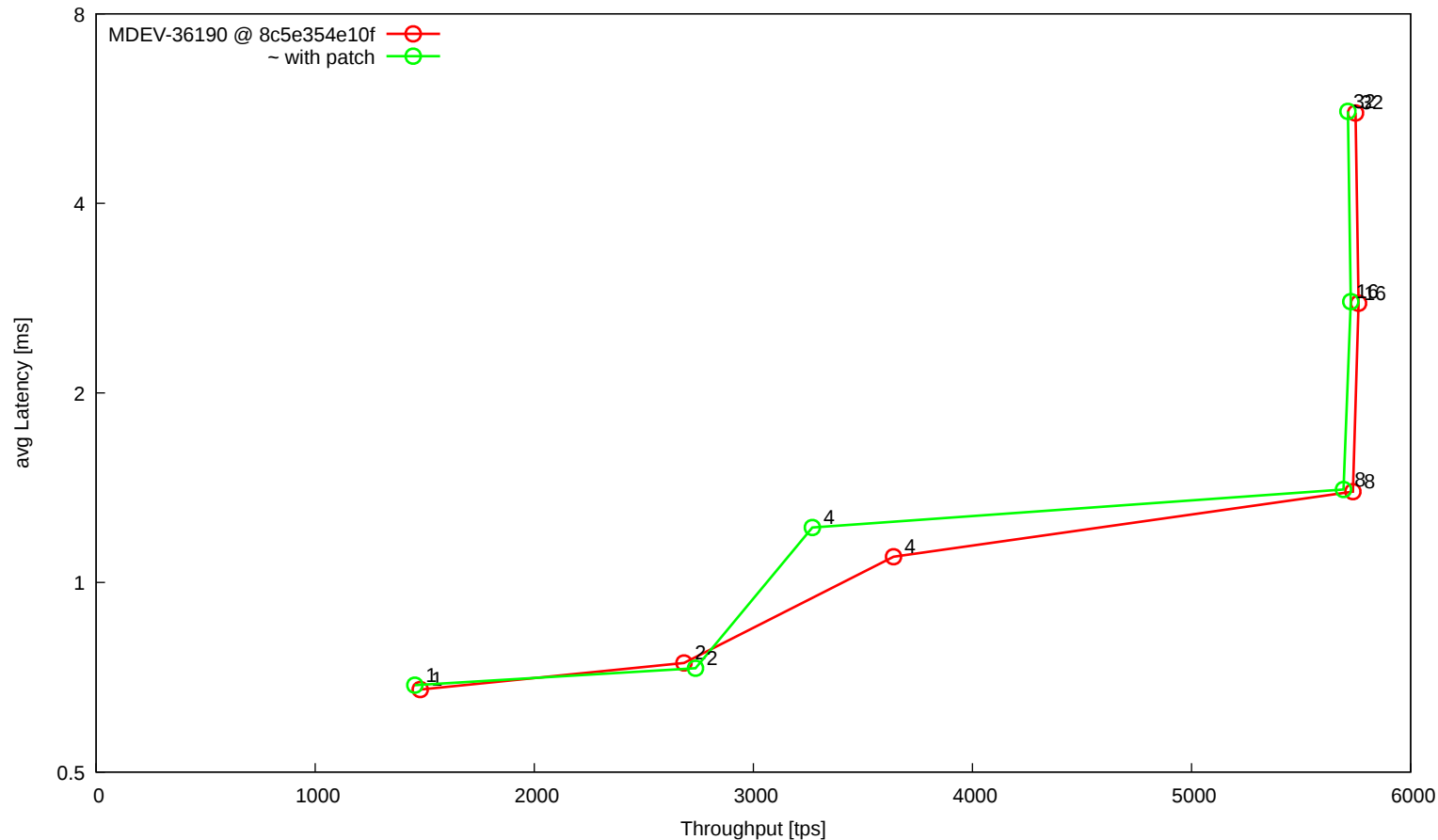
t_oltp_order_big_ranges
