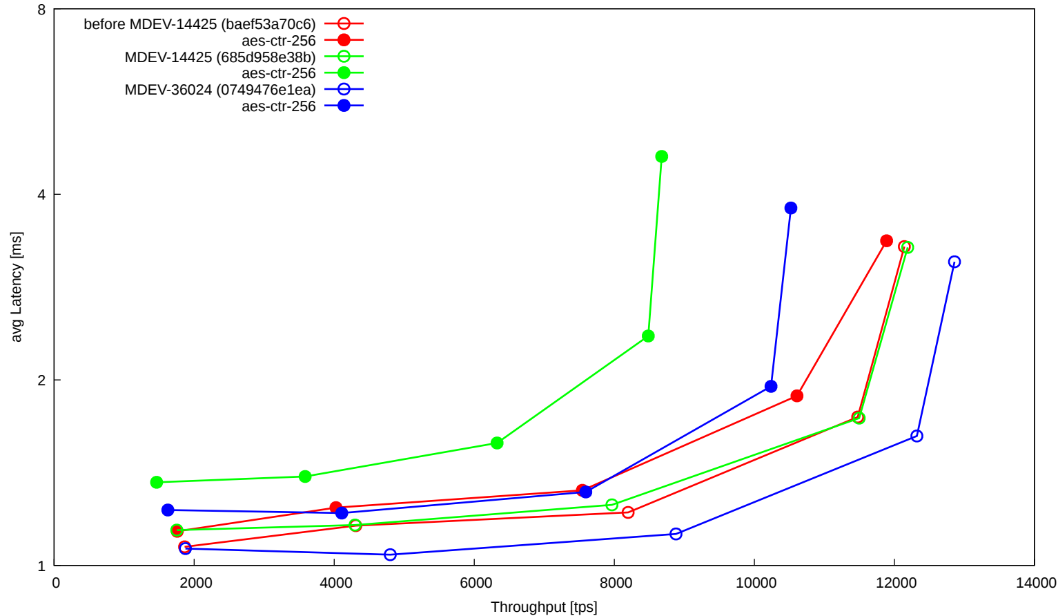
InnoDB OLTP INSERTs (10 per TRX) with and without InnoDB encryption
