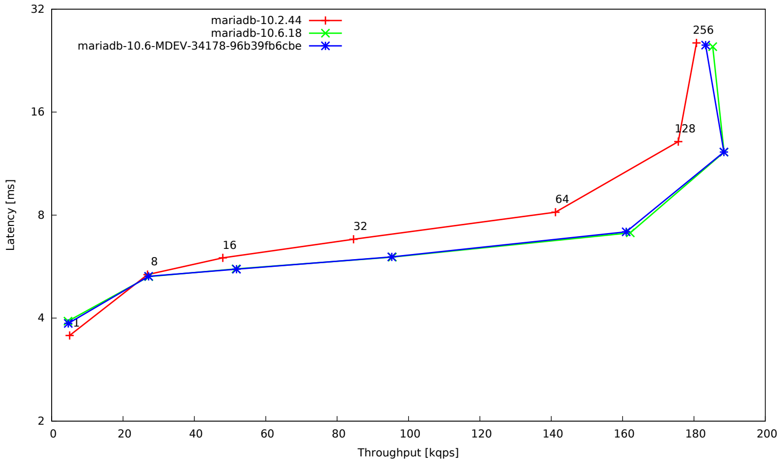
t_oltp-innodb-multi-2
