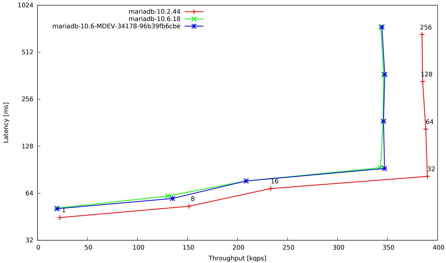
t_1K-reads-memory-multi
