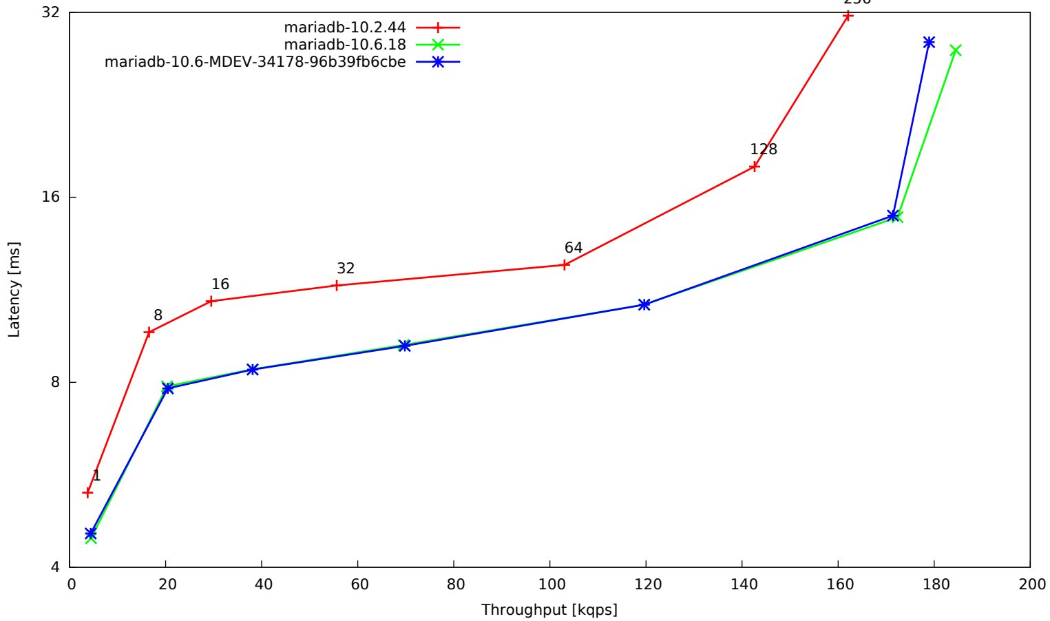
t_writes-binlog-multi-2
