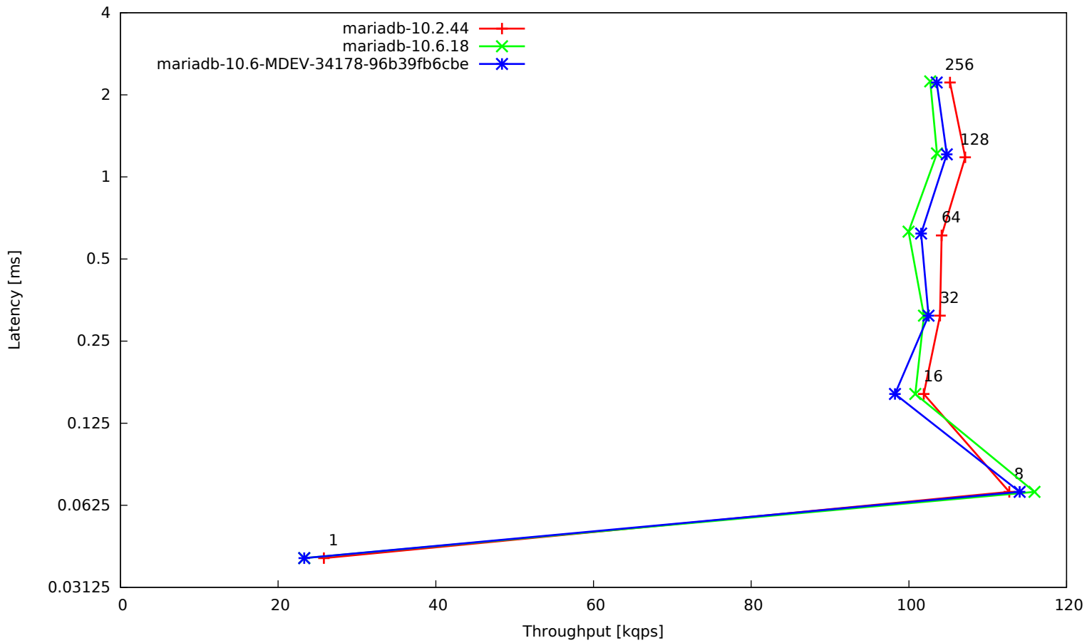
t_insert-memory-multi
