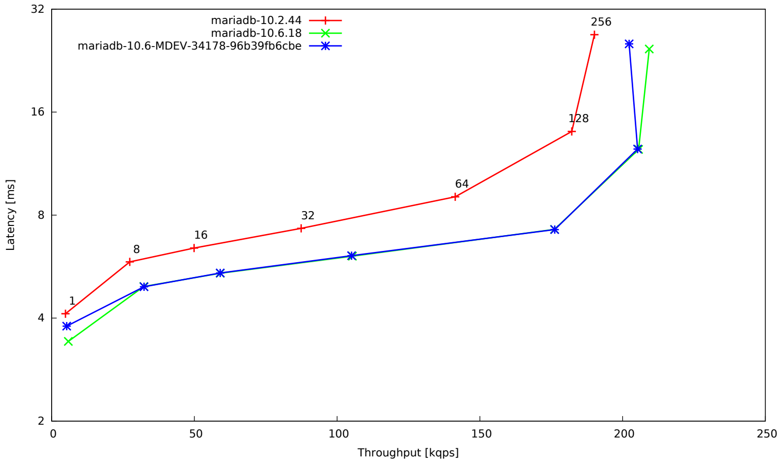
t_writes-innodb-multi-2
