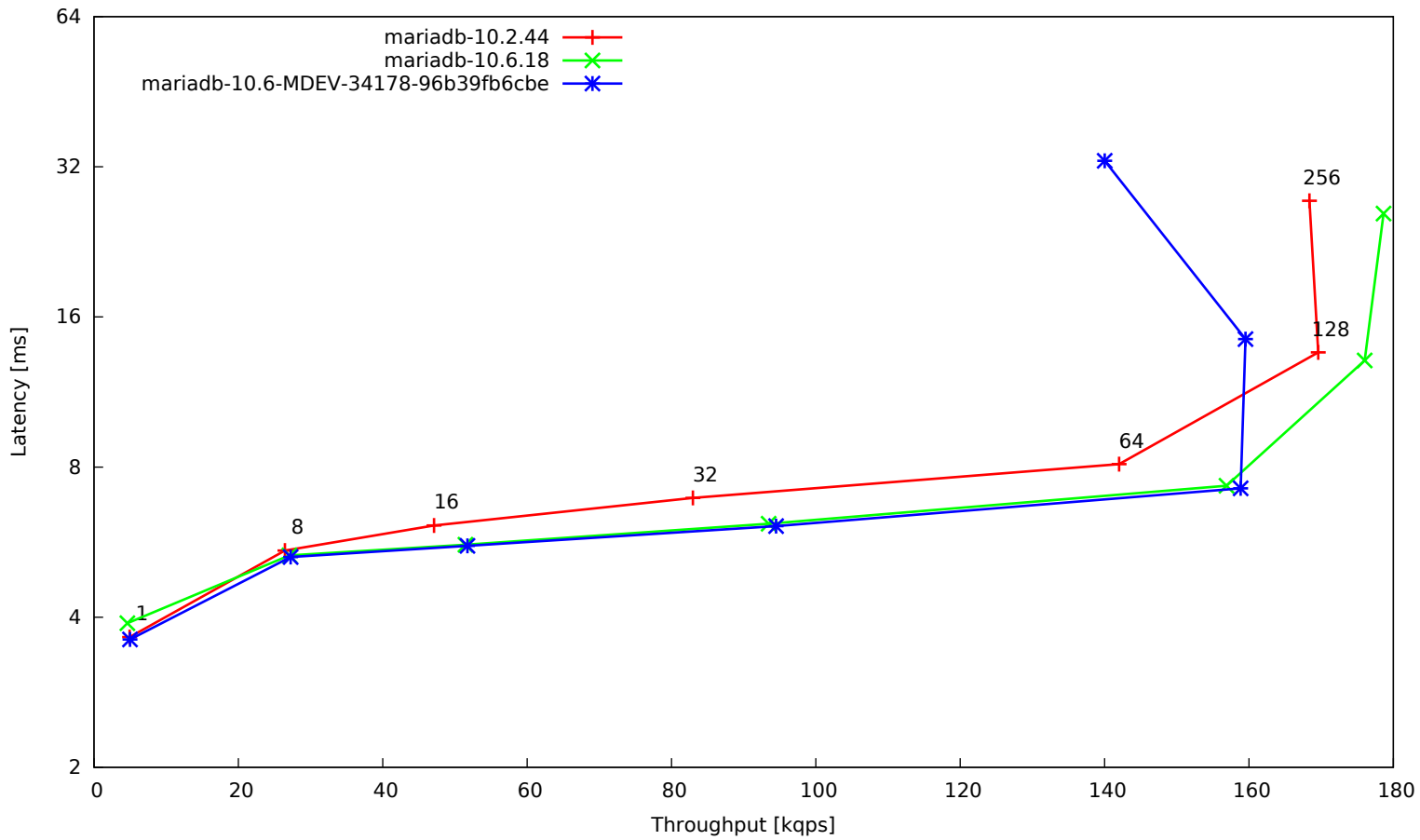
t_oltp-innodb-single-2
