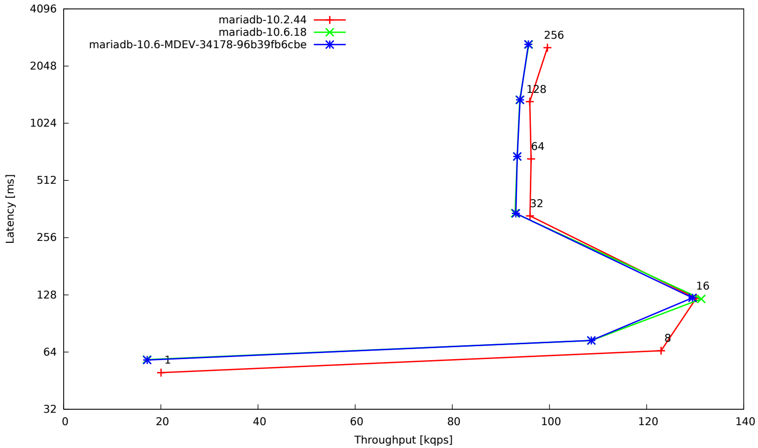
t_1K-reads-mysam-single
