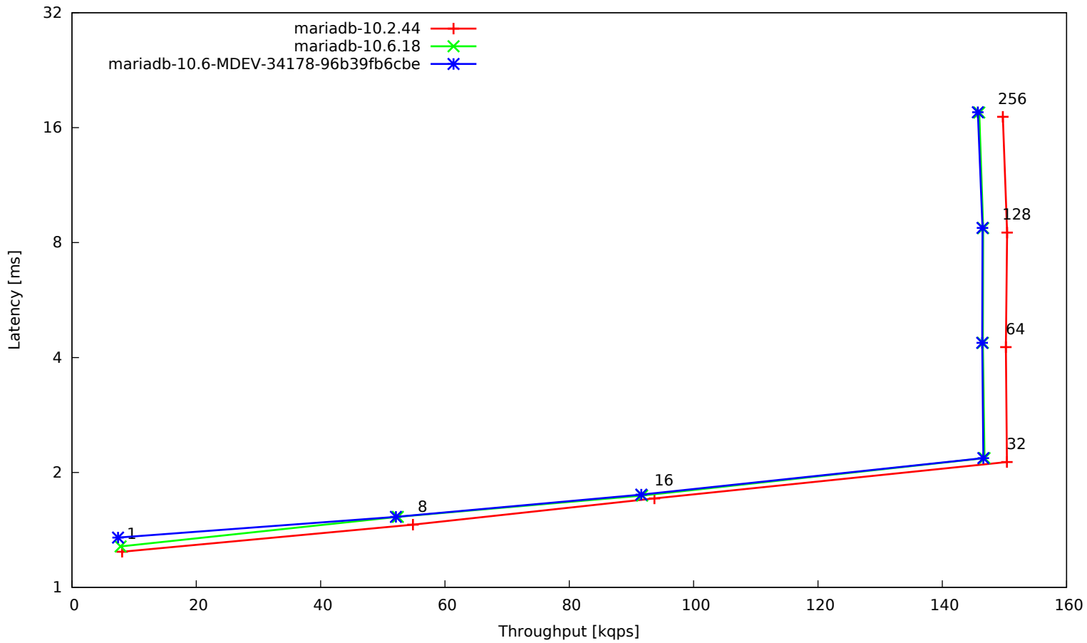
t_collate_distinct_range_utf8_general
