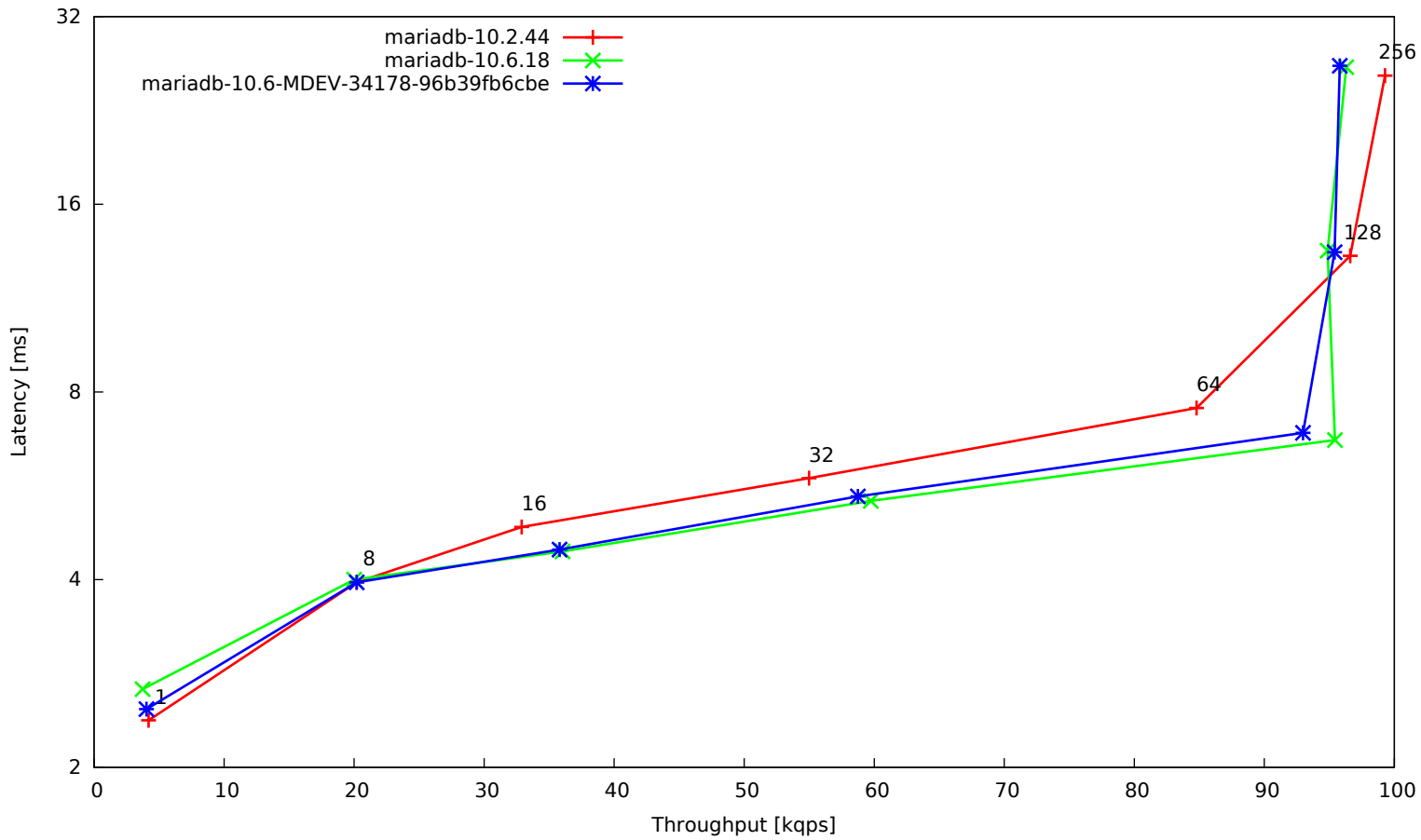
t_insert-batched-innodb-multi
