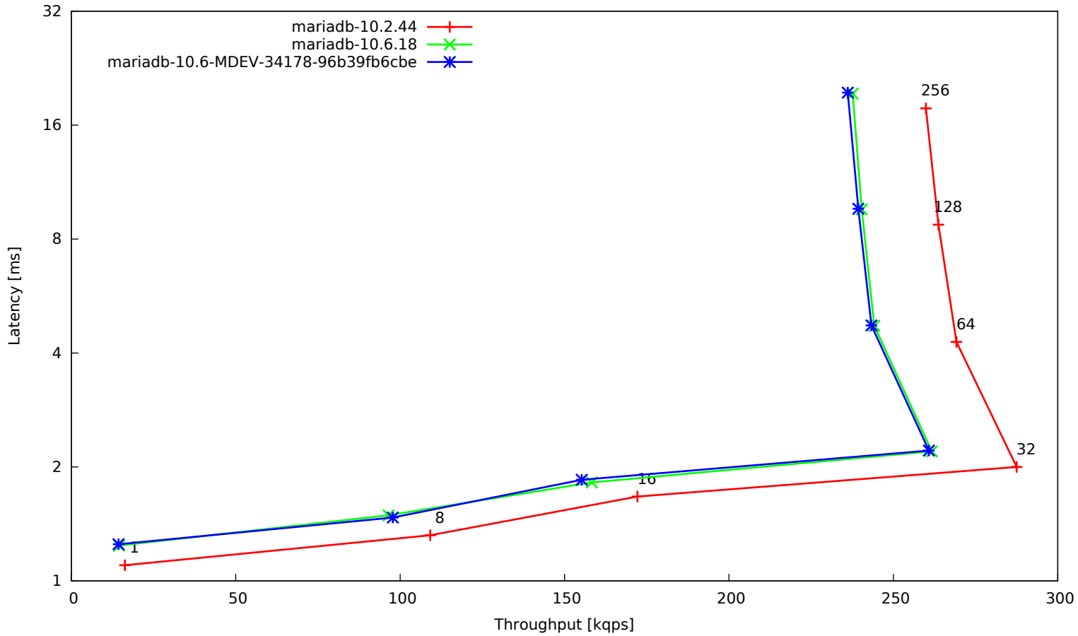
t_oltp-memory-btree-multi
