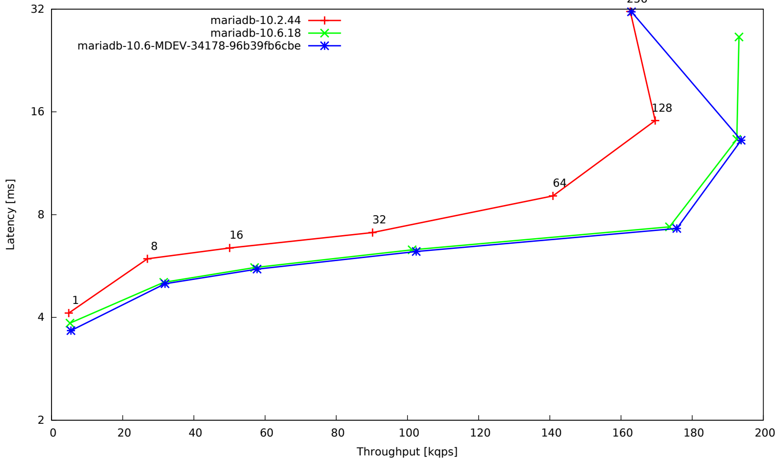
t_writes-innodb-single-2
