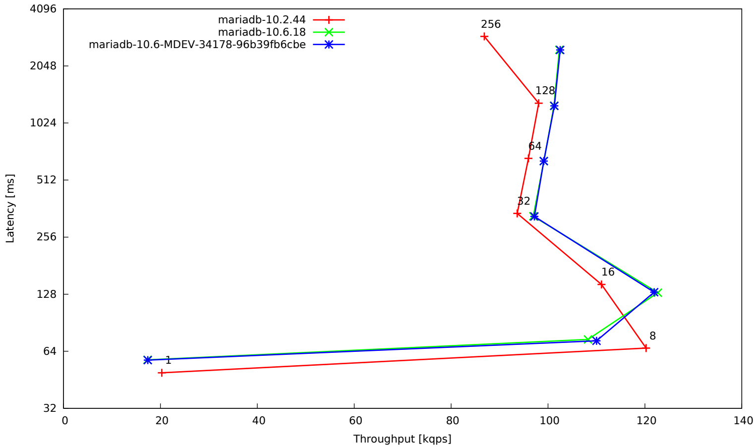
t_1K-reads-aria-multi
