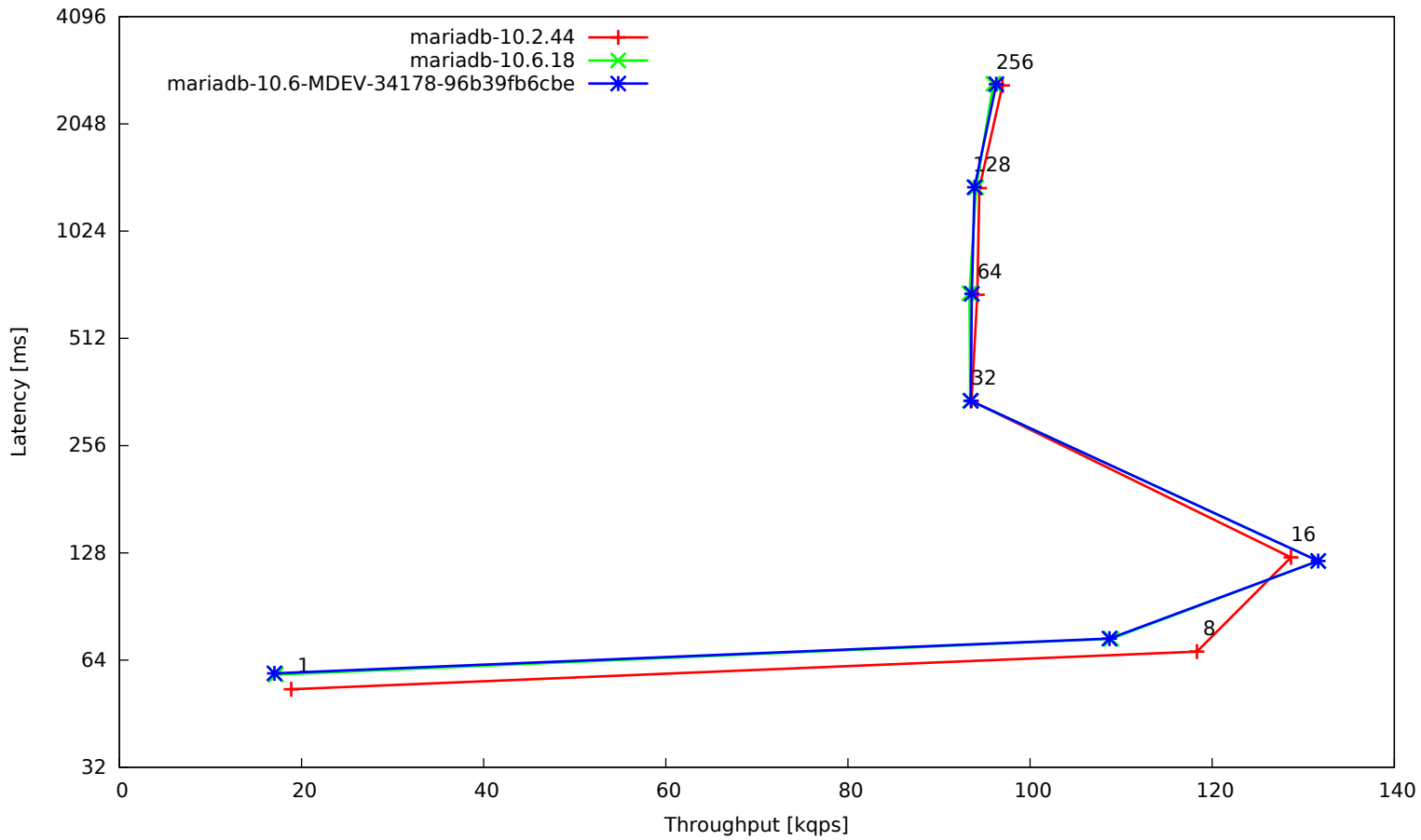
t_1K-reads-myisam-multi
