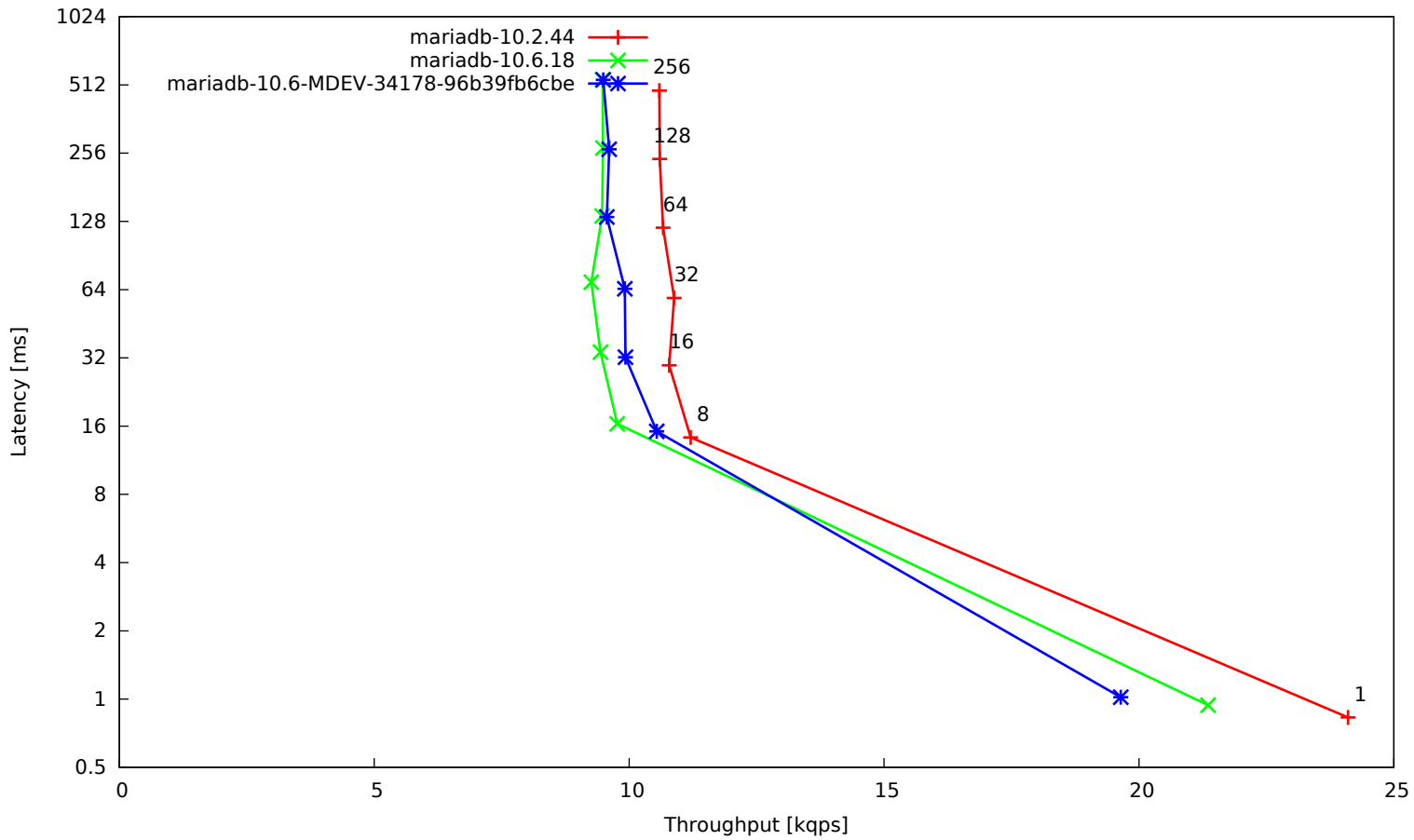
t_writes-memory-single
