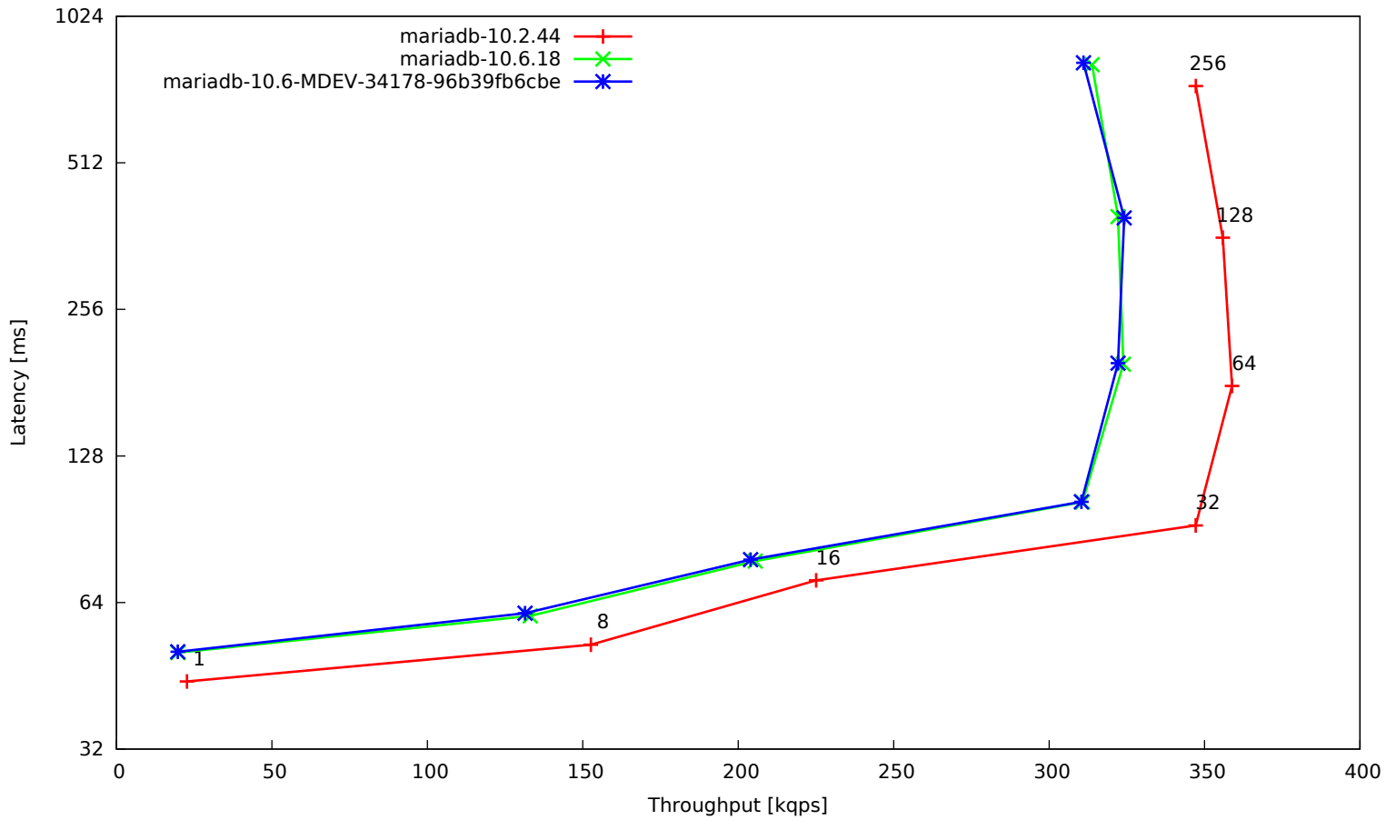
t_1K-reads-memory-single
