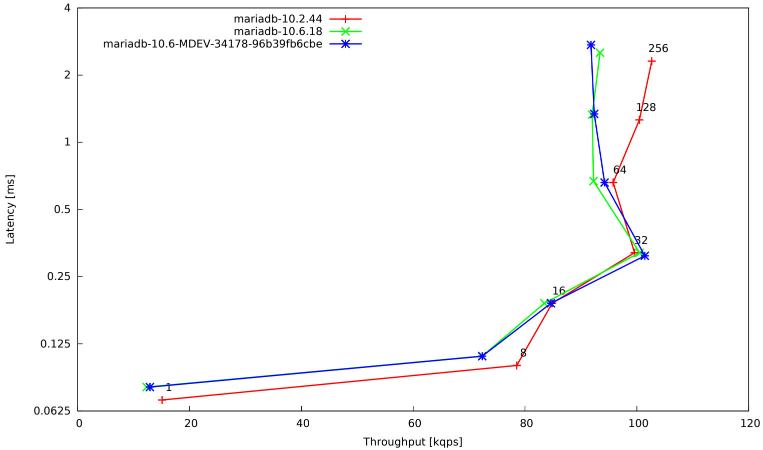
t_insert-innodb-multi
