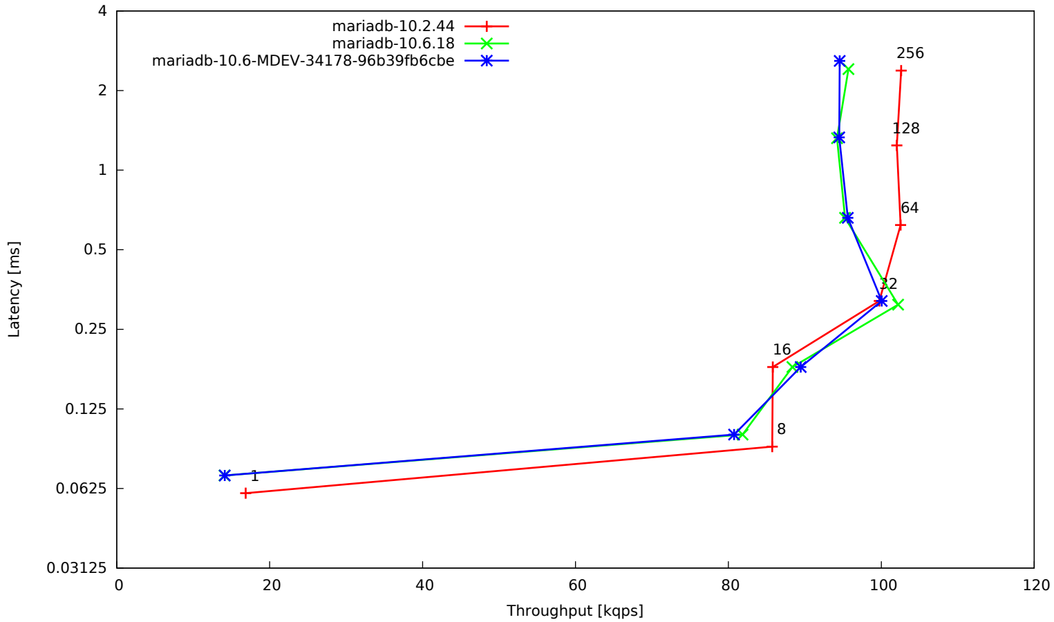
t_insert-innodb0-multi
