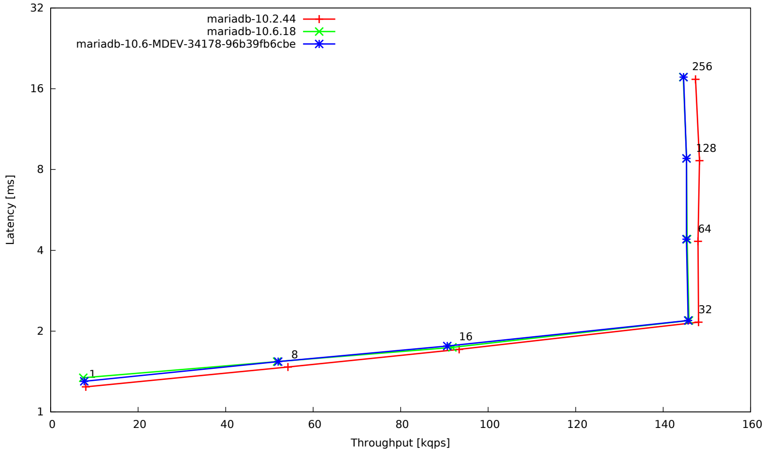
t_collate_distinct_range_utf8mb4_general
