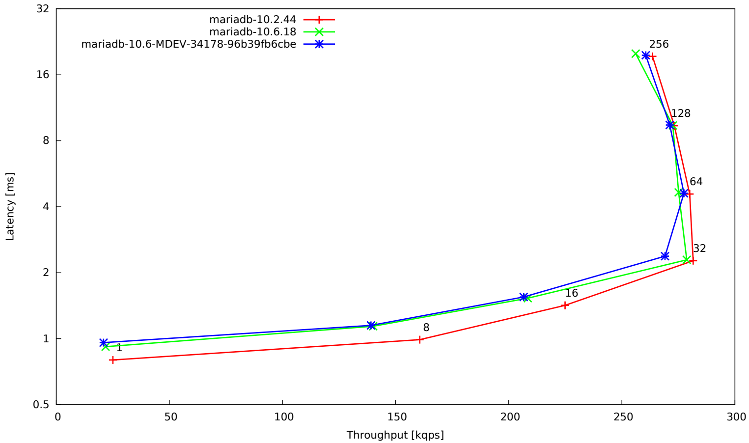
t_writes-memory-multi
