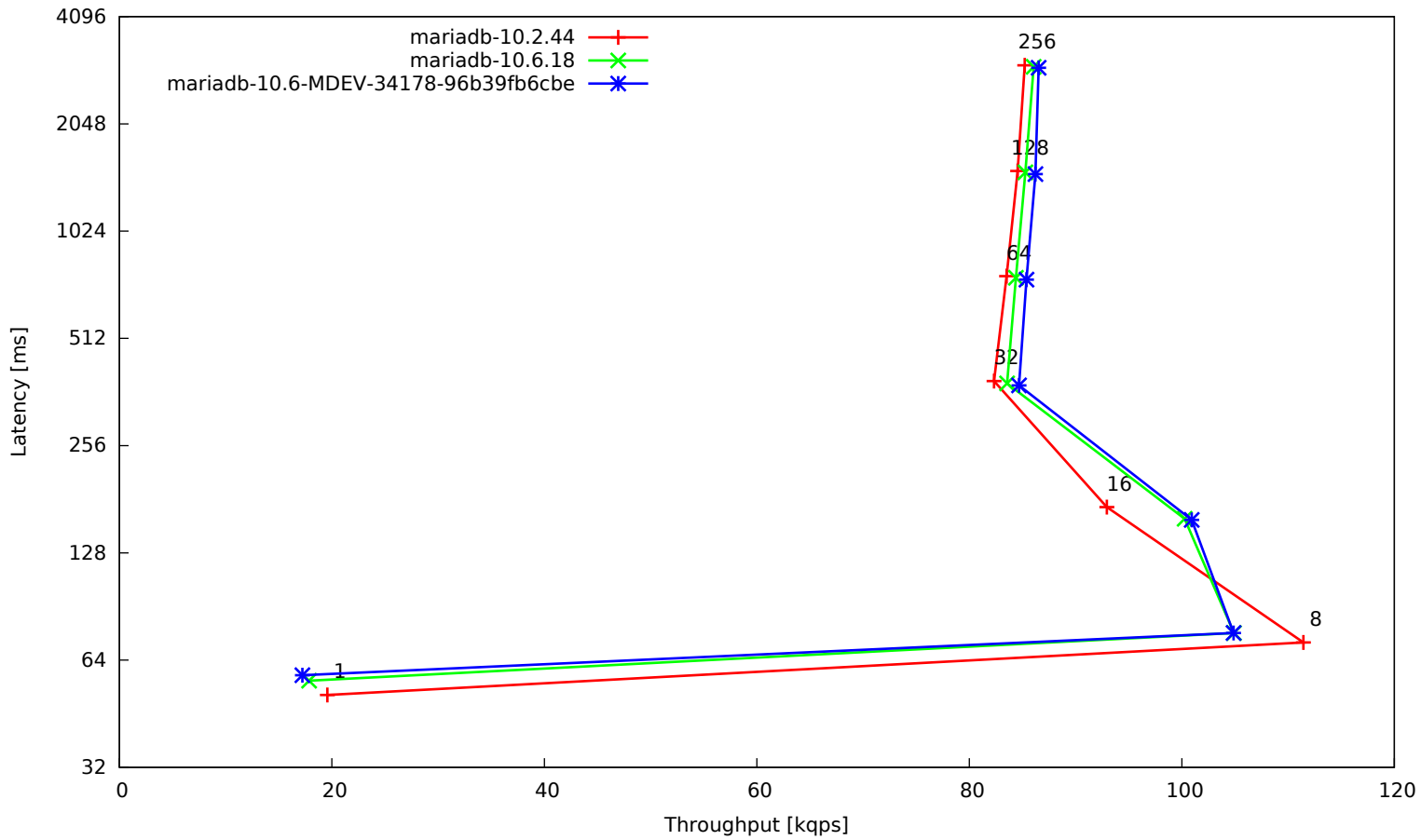
t_1K-reads-aria-single
