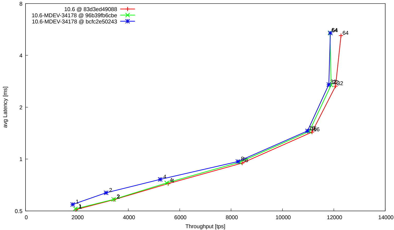
t_oltp_insert_innodb_batched
