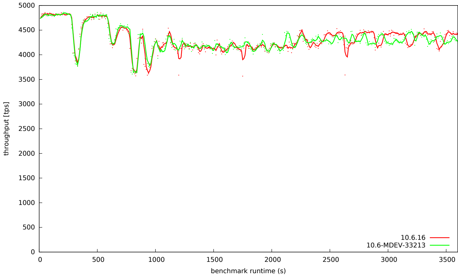
sysbench tpcc, scale 32x5, 32 threads, innodb_undo_log_truncate = ON
