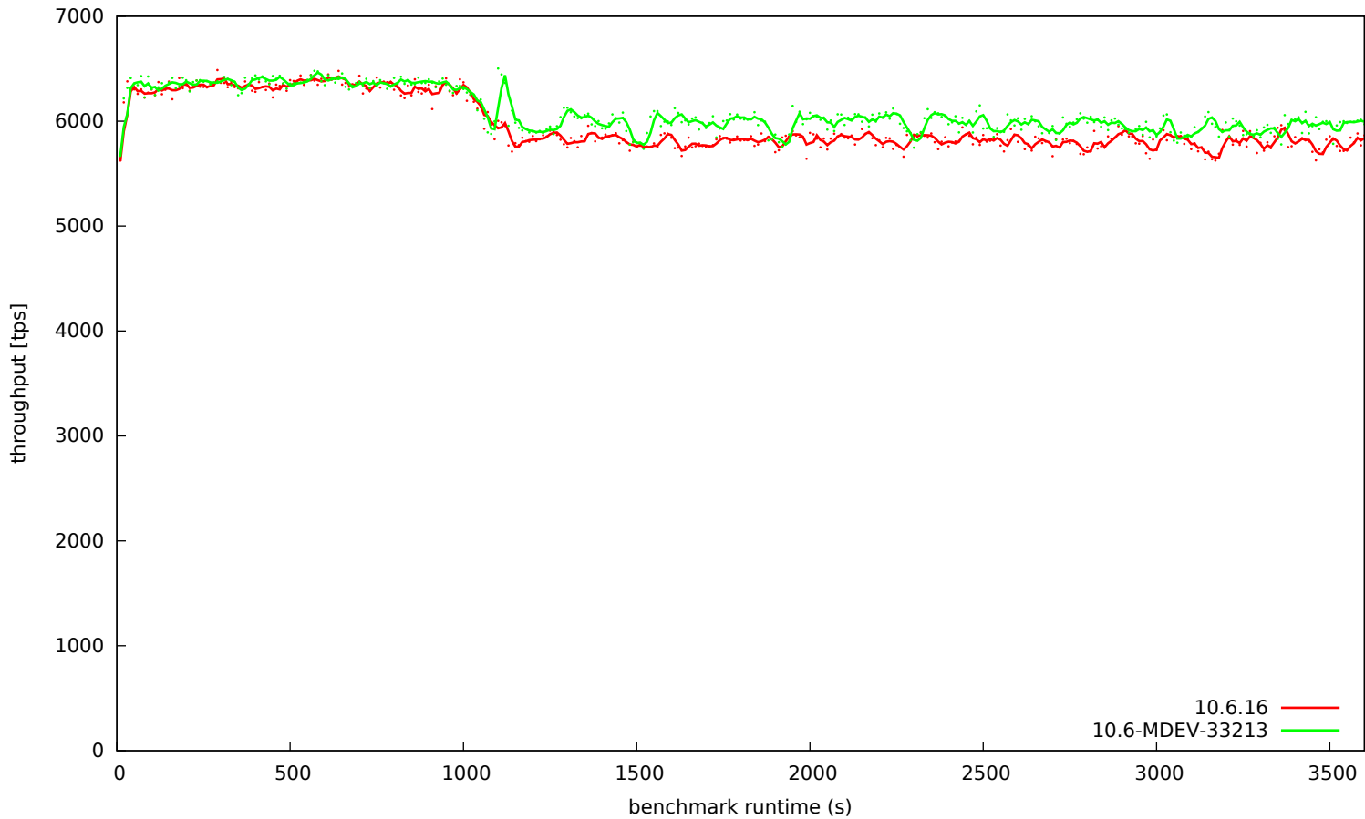
sysbench tpcc, scale 64x5, 64 threads
