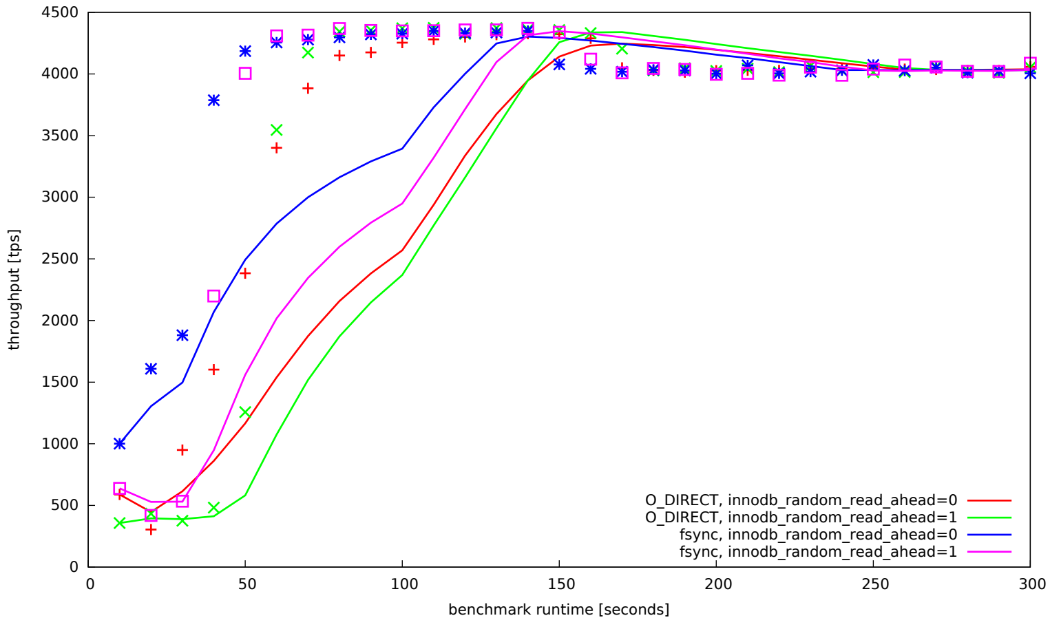
sysbench tpcc, scale 64x10, 64 threads, 64G BP, SSD, 10.6 HEAD (commit 691e964d235)
