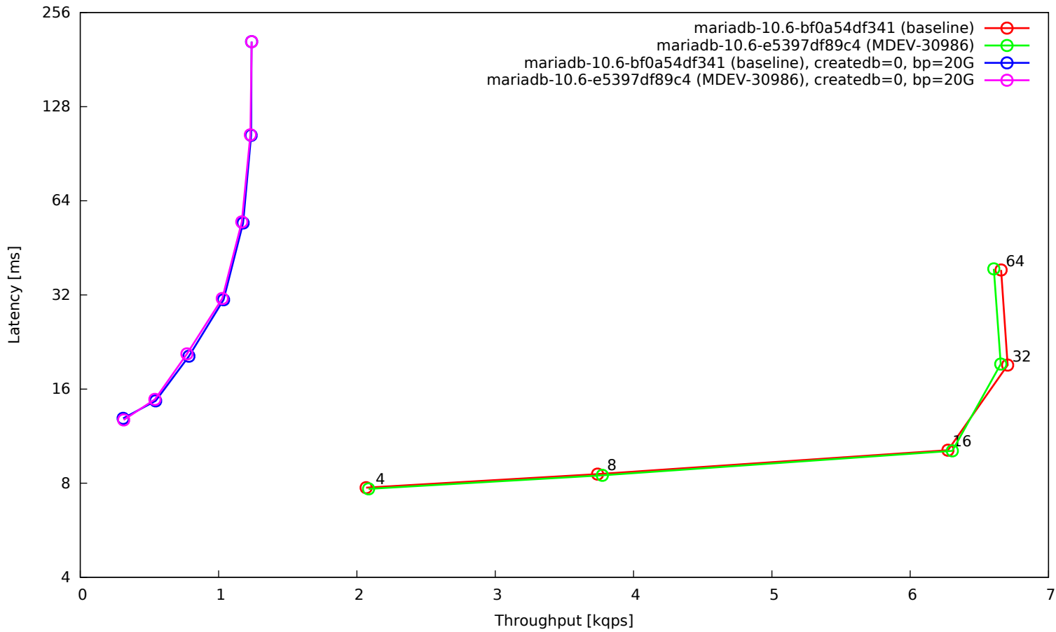
OLTP read-only w/ long range scans, 16 tables, 30G data set, 32G buffer pool, SSD
