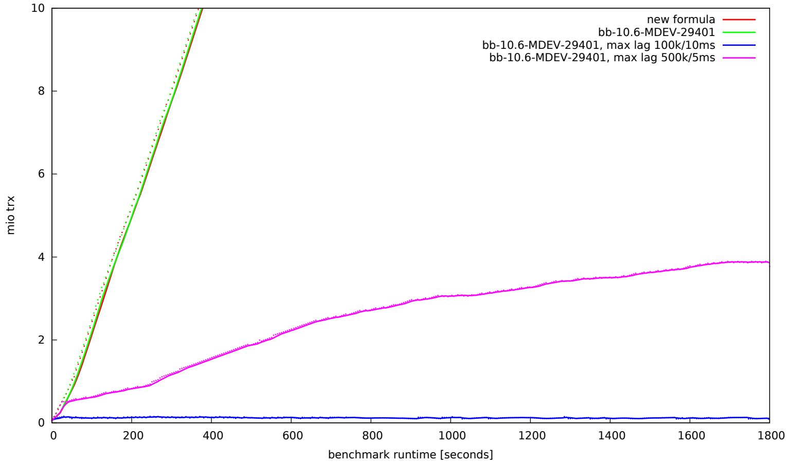
history list length, 512 threads, 32G data set, 64G BP, SSD, lwm=10
