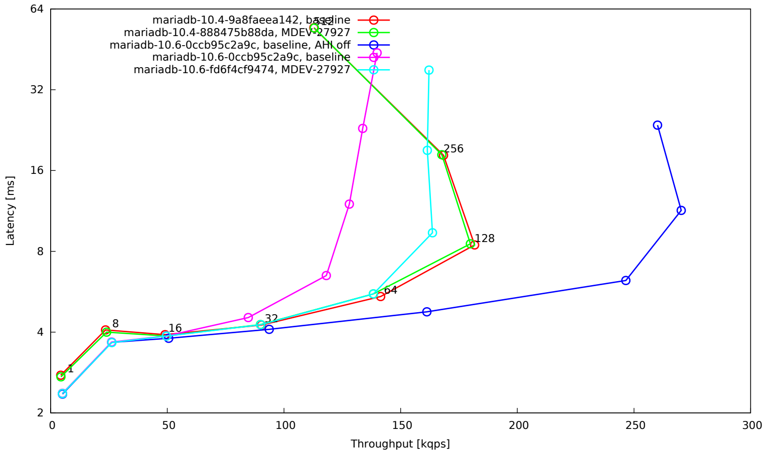
OLTP update indexed column (10 per trx), 16 tables with 100K rows each, 32G buffer pool, SSD
