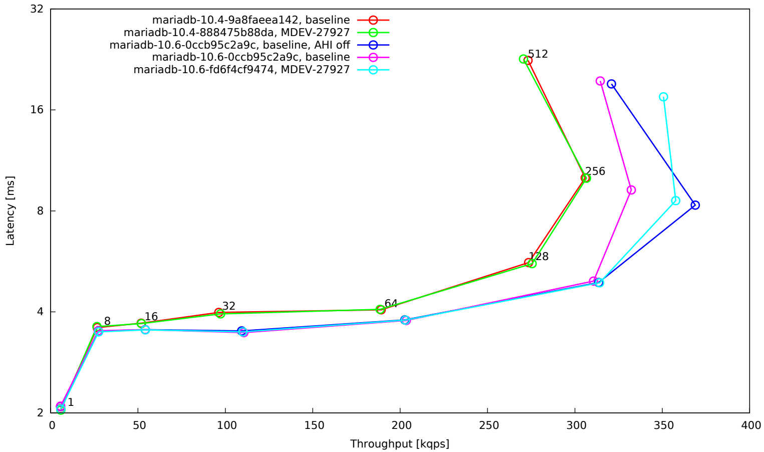
OLTP read/write 90:10, 16 tables with 100K rows each, 32G buffer pool, SSD
