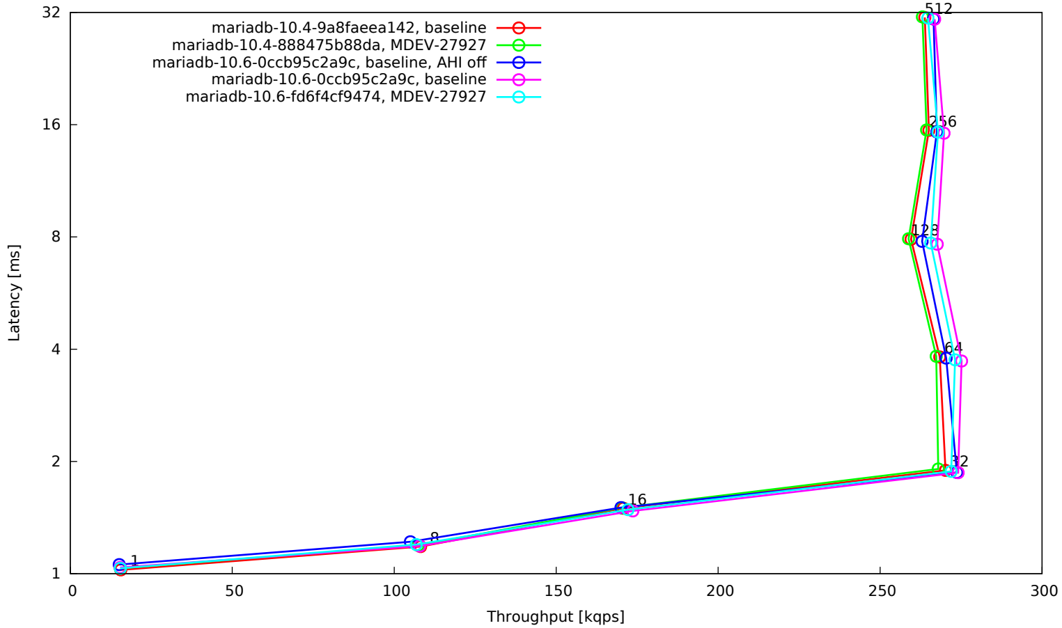
OLTP read-only default mix, 16 tables with 100K rows each, 32G buffer pool, SSD
