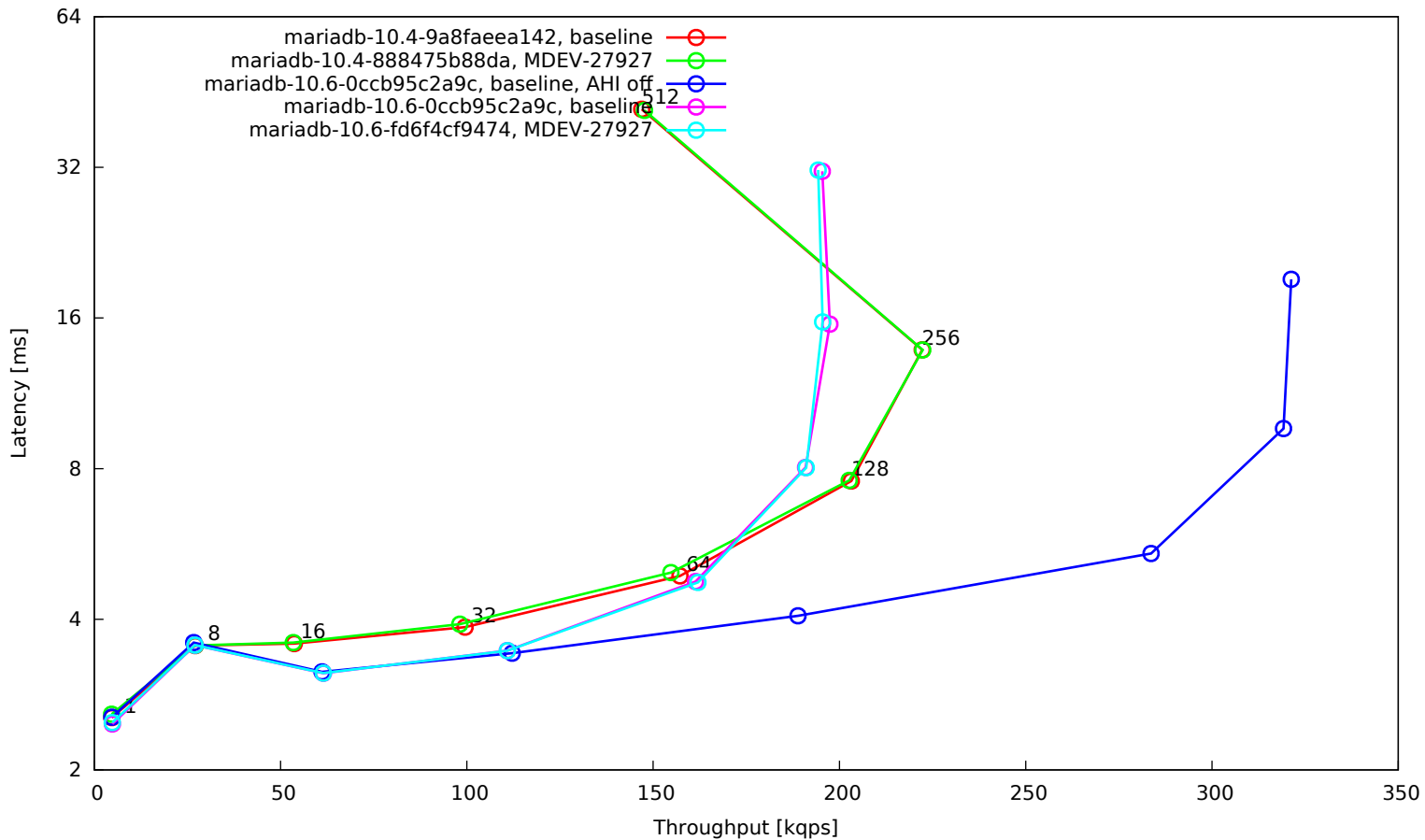
OLTP update unindexed column (10 per trx), 16 tables with 100K rows each, 32G buffer pool, SSD
