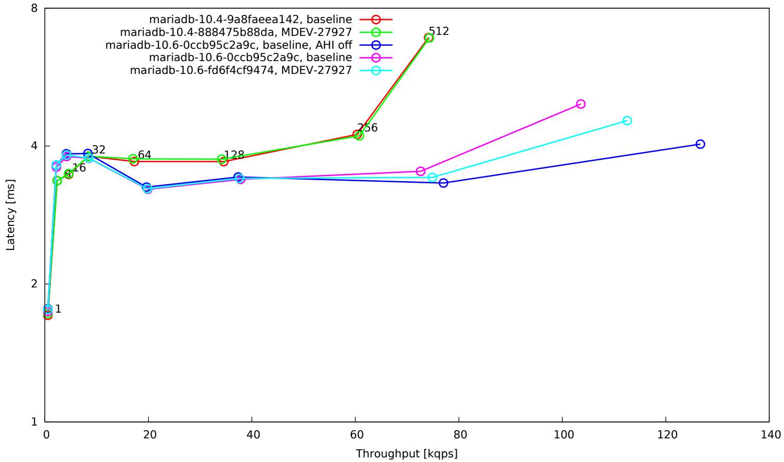
OLTP update indexed column, 16 tables with 100K rows each, 32G buffer pool, SSD
