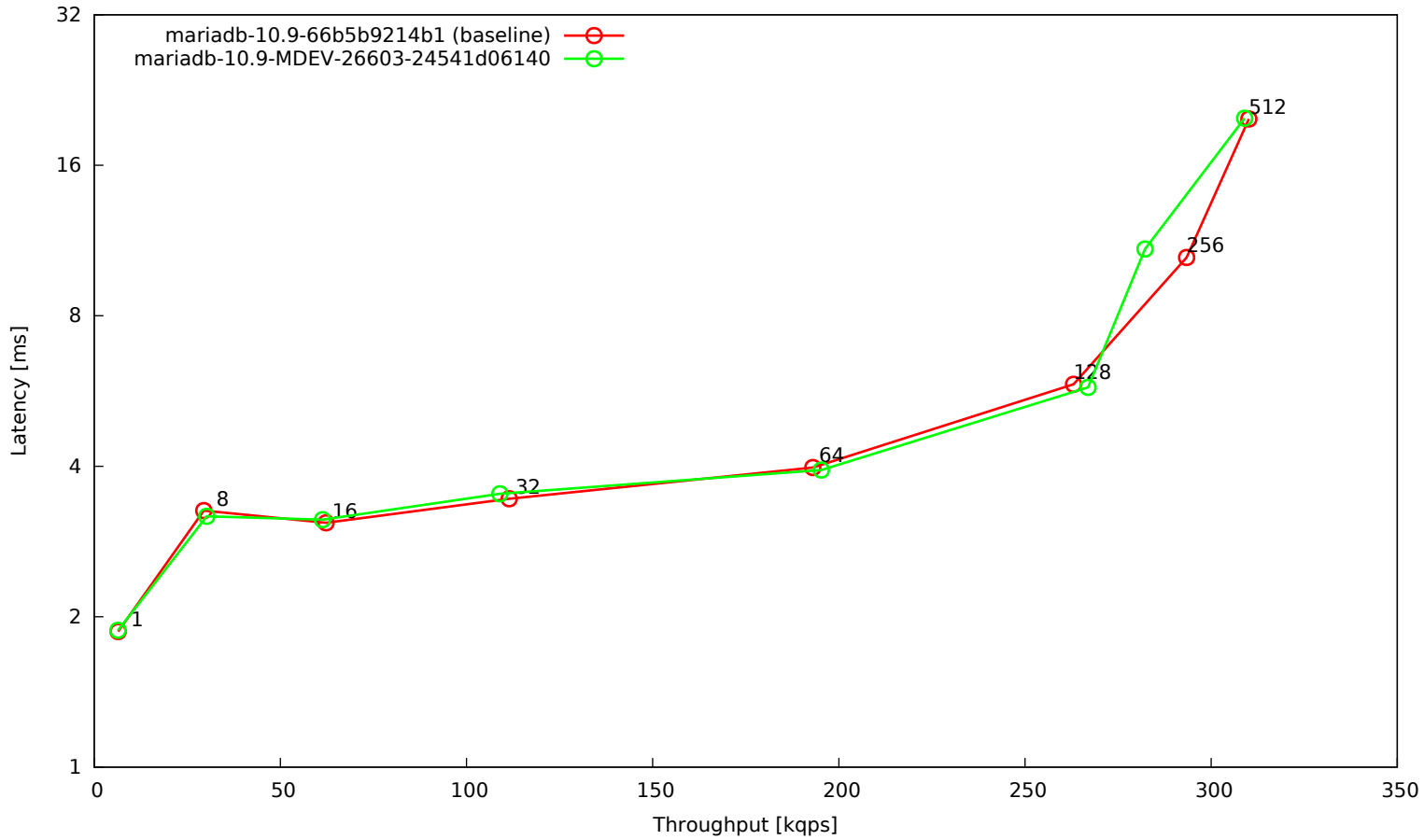
OLTP update unindexed column (10 per trx), 16 tables, 4G data set, 32G buffer pool, SSD
