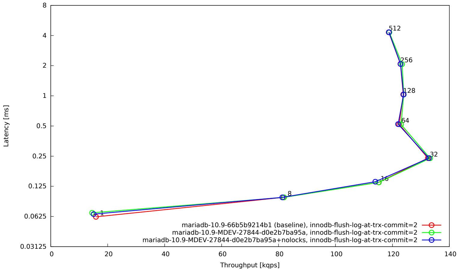
OLTP insert (no autoinc), 16 tables, 4G data set, 32G buffer pool, SSD
