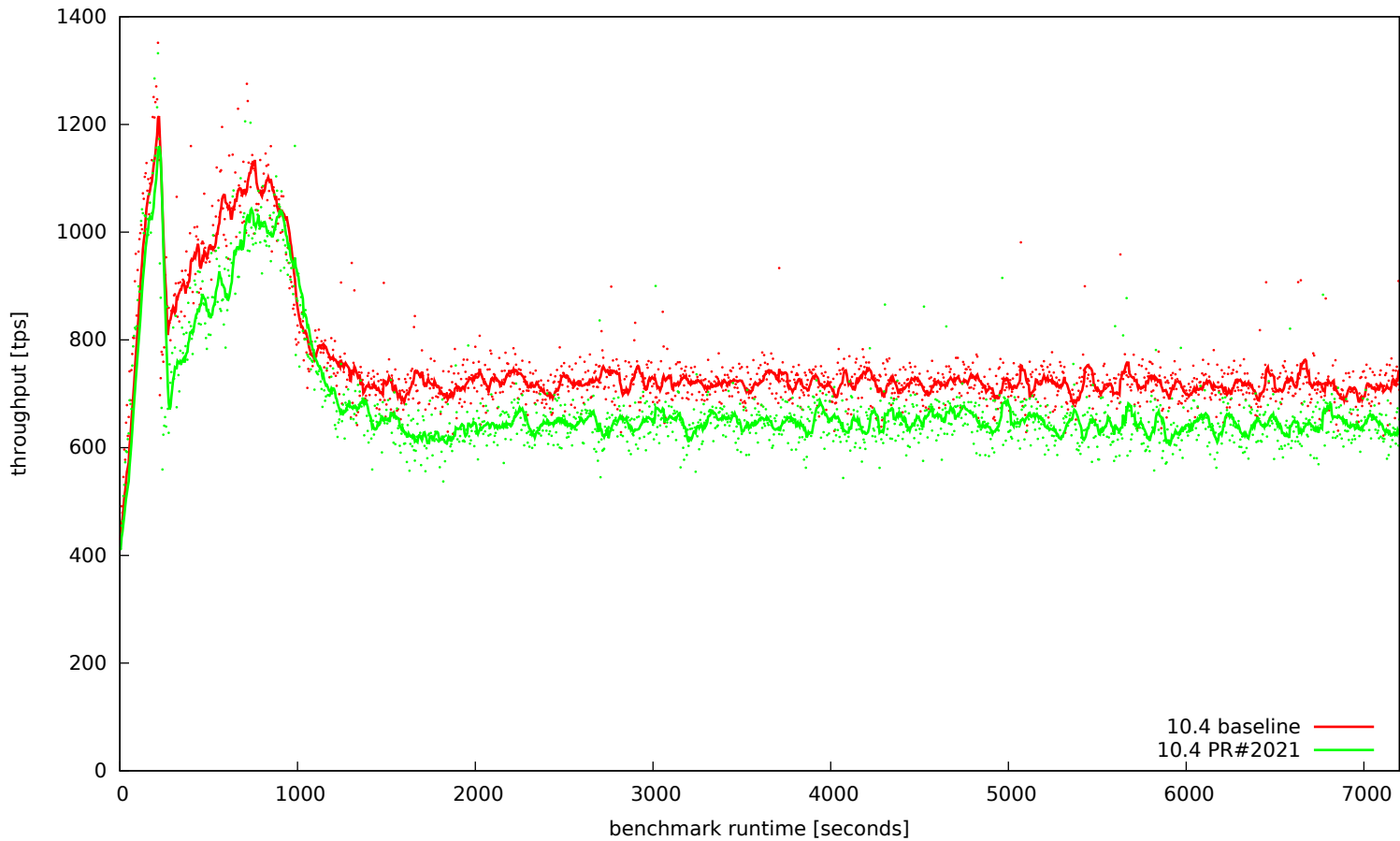
sysbench tpcc, scale 1600, 32 threads, 80G BP, SSD
