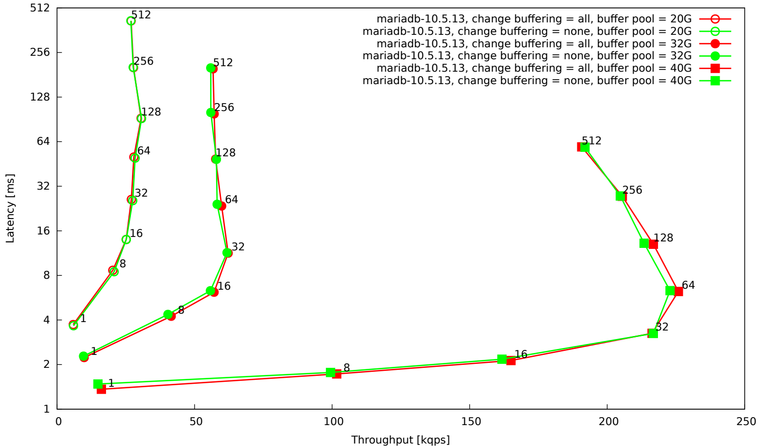
OLTP tables, 10 point-selects using SK, 1 delete+insert, 16 tables, 160 mio rows
