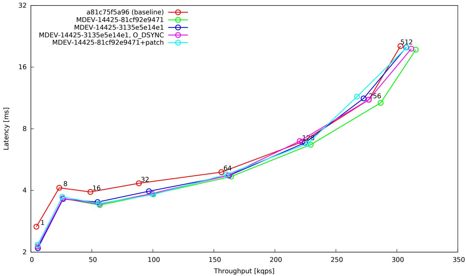
OLTP update unindexed column (10 per trx), 16 tables, 8G data set, 32G buffer pool, SSD
