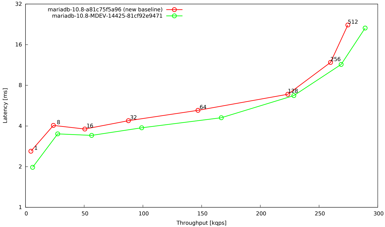
OLTP update unindexed column (10 per trx), 16 tables, 8G data set, 32G buffer pool, SSD
