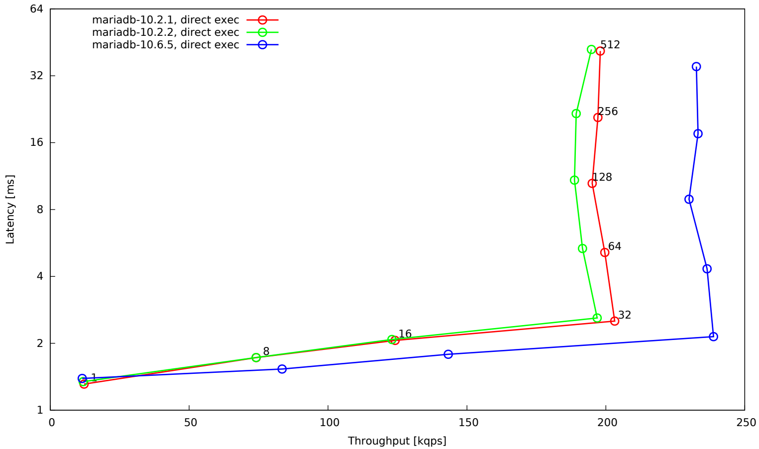
OLTP read-only, 32 tables, 1 mio rows each, big BP, SSD
