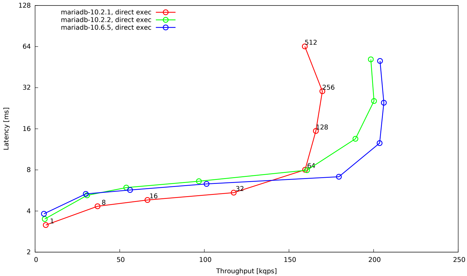
OLTP read/write default mix, 32 tables, 1 mio rows each, big BP, SSD
