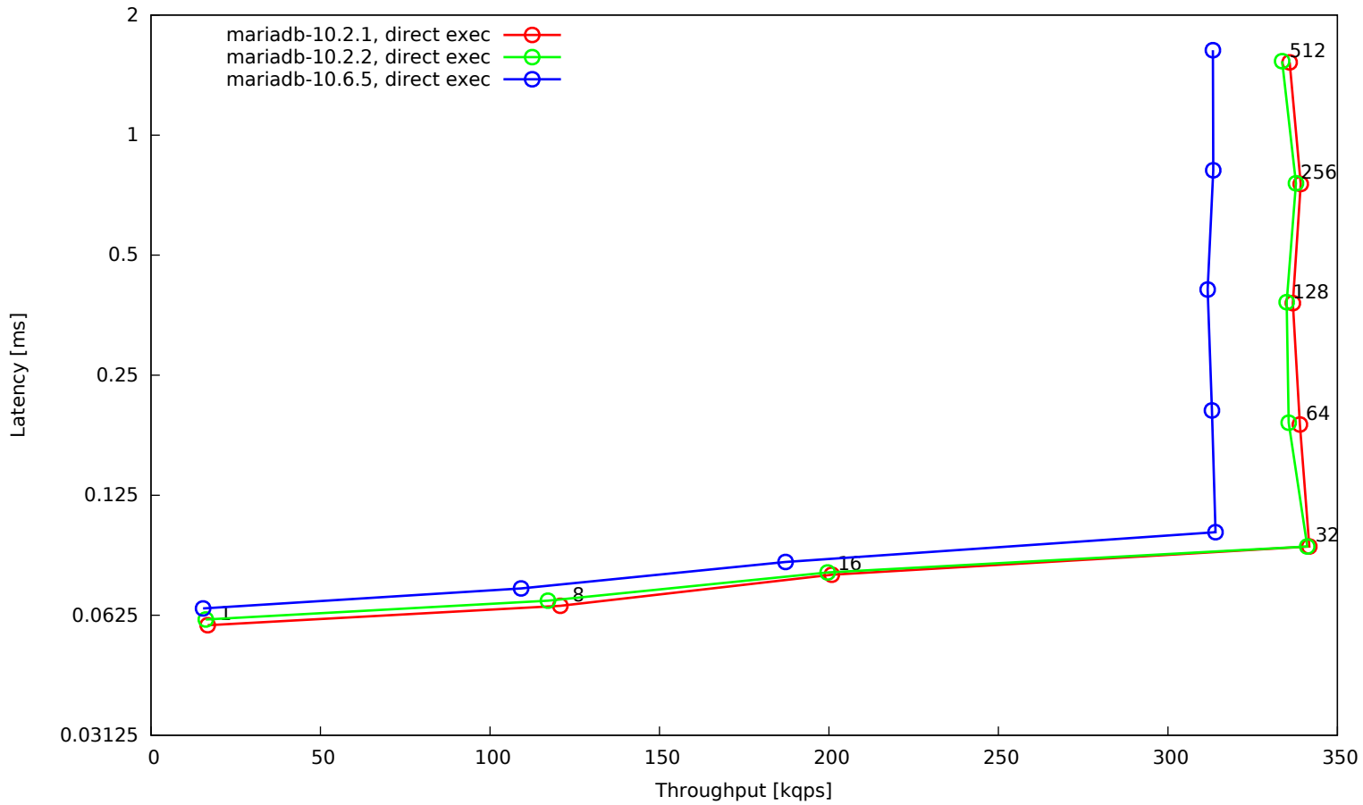
OLTP point selects (no TRX), 32 tables, 1 mio rows each, big BP, SSD
