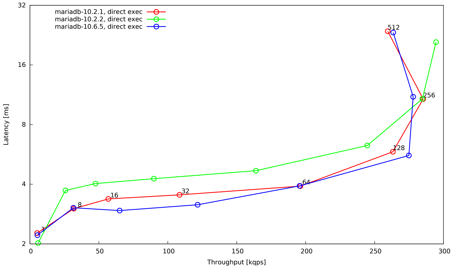
OLTP read/write 90:10, 32 tables, 1 mio rows each, big BP, SSD
