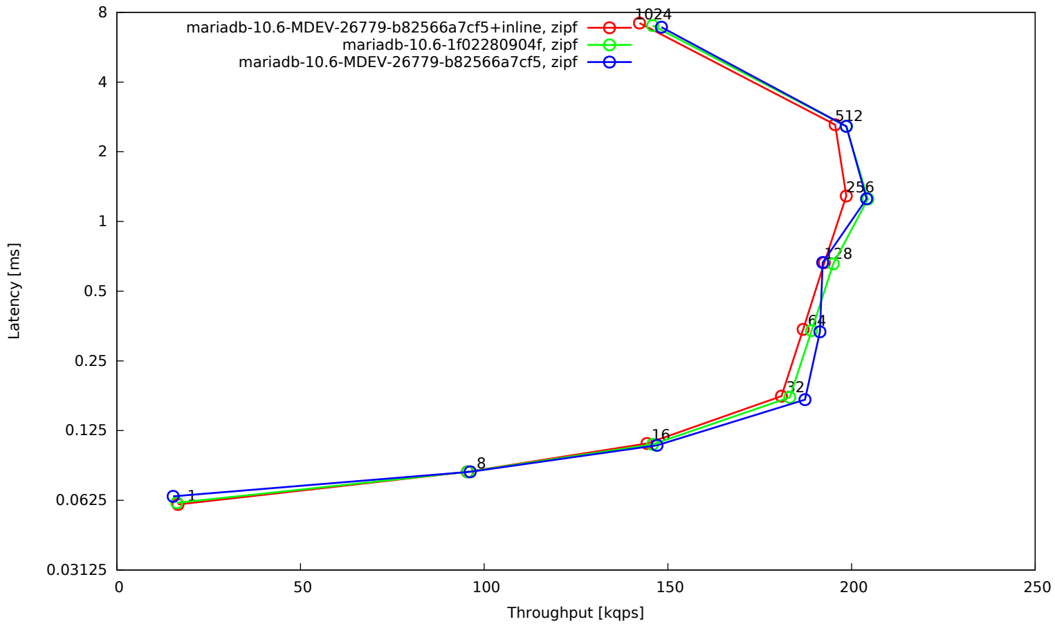
OLTP update unindexed column, 16 tables, 2 mio rows each, big BP, RAM disk
