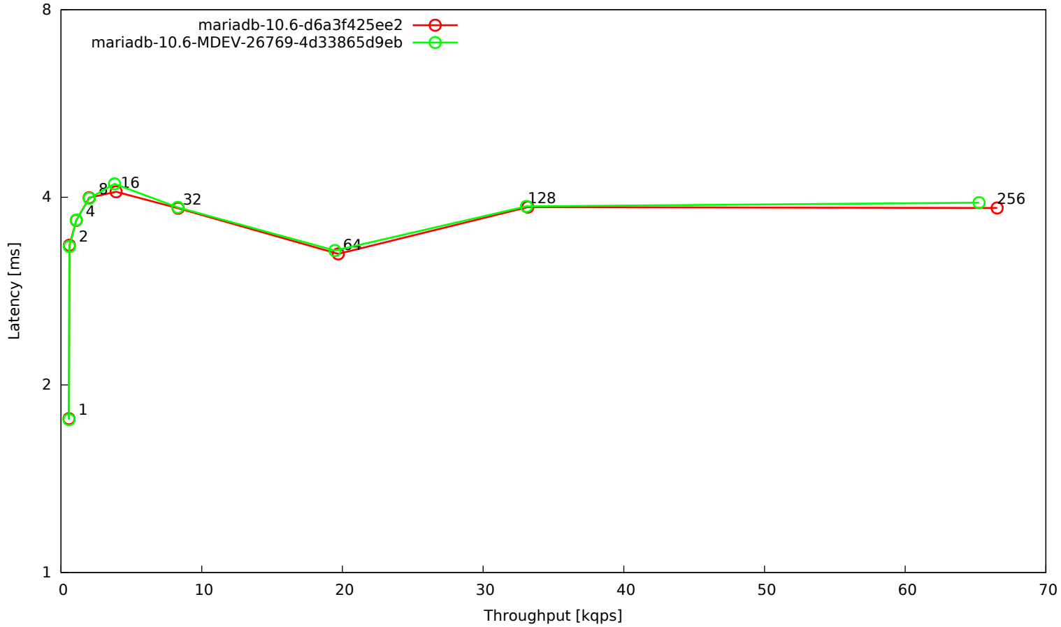
OLTP update unindexed column, 16 tables, 2 mio rows each, big BP, RAM disk
