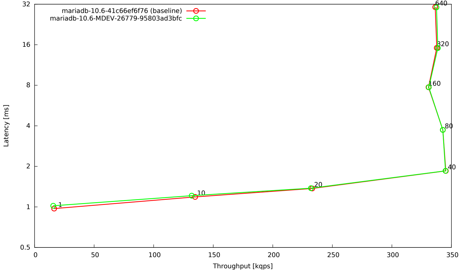
OLTP read-only, 20 tables, 2 mio rows each, big BP, NVMe disk
