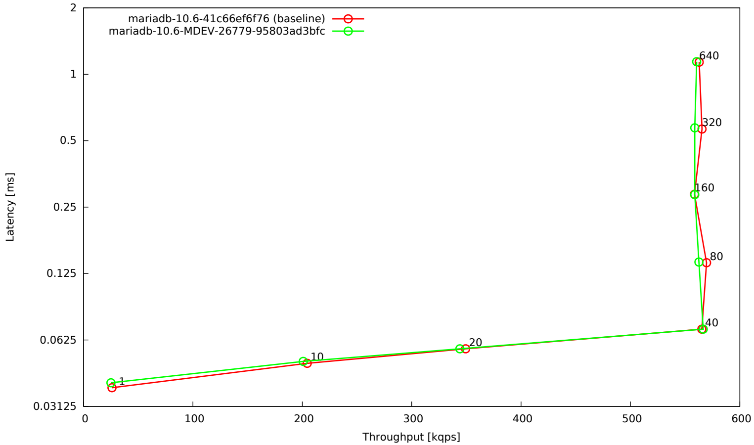
OLTP point selects, 20 tables, 2 mio rows each, big BP, NVMe disk
