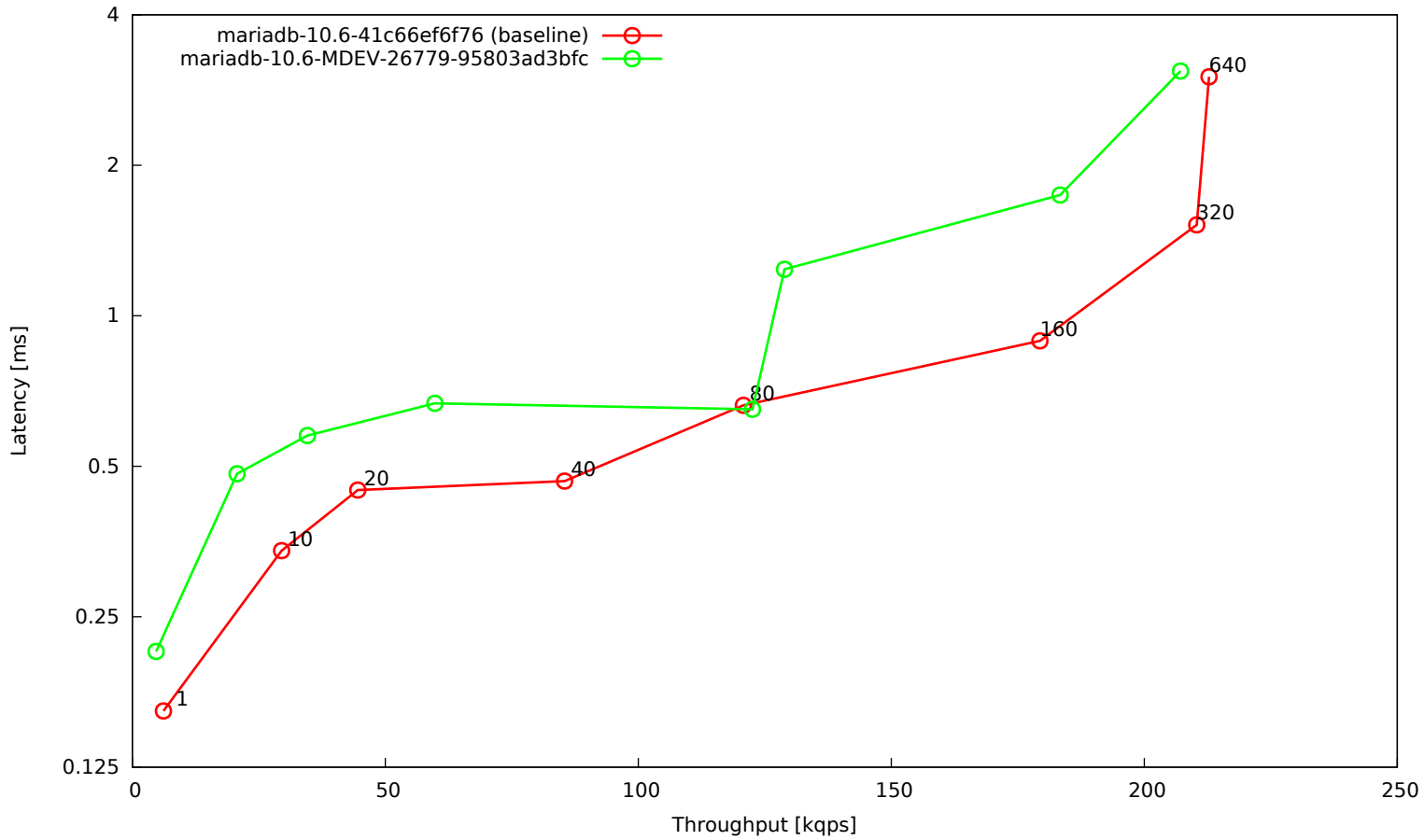
OLTP update unindexed column, 20 tables, 2 mio rows each, big BP, NVMe disk
