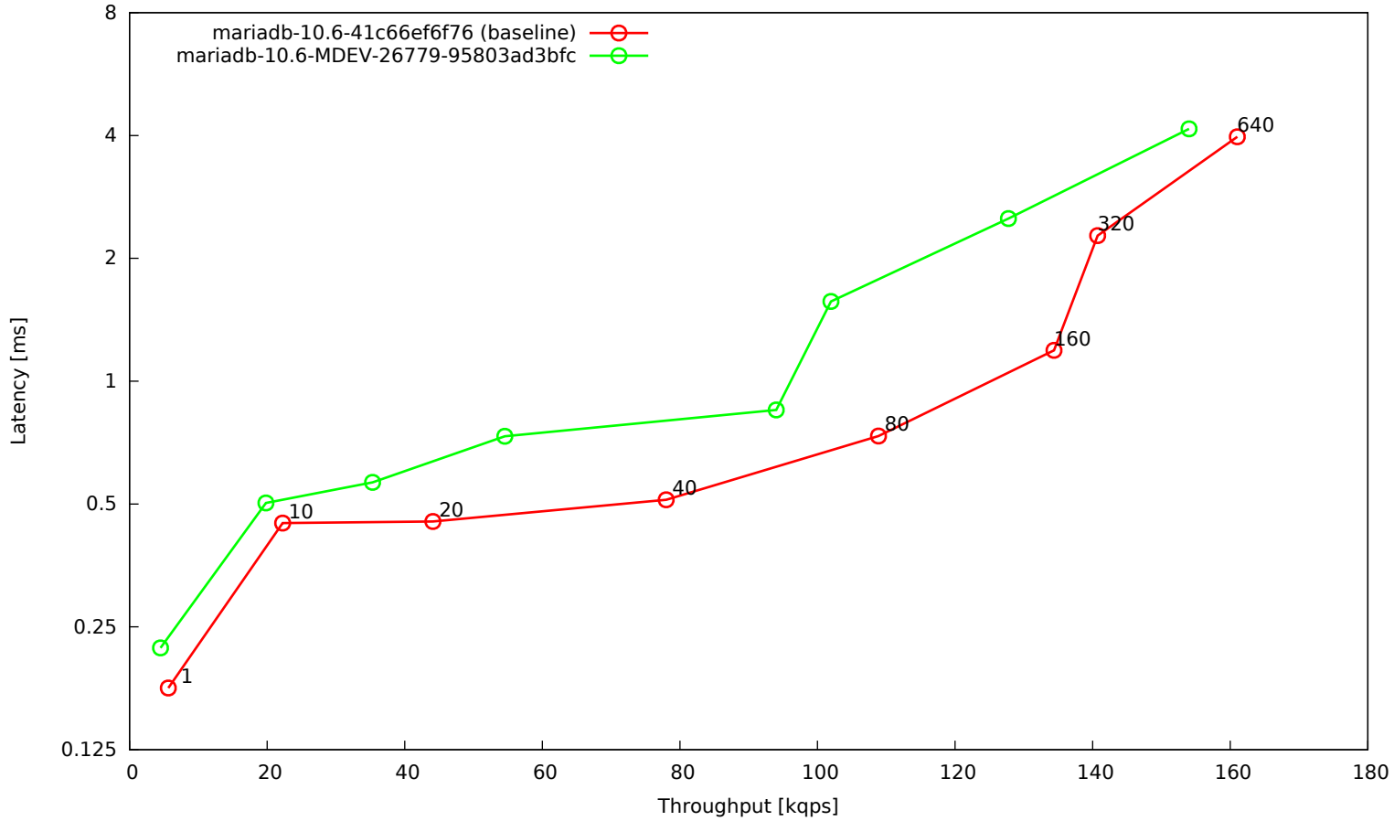
OLTP update indexed column, 20 tables, 2 mio rows each, big BP, NVMe disk
