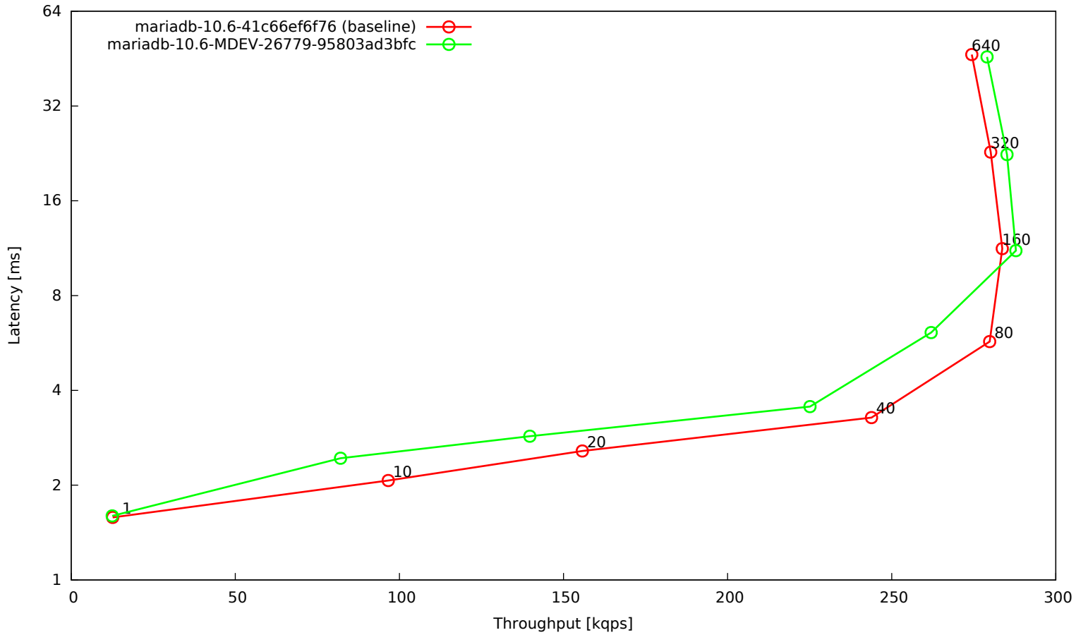
OLTP read/write default mix, 20 tables, 2 mio rows each, big BP, NVMe disk
