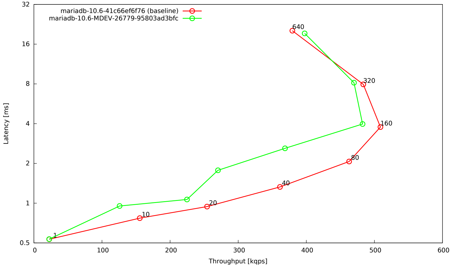
OLTP read/write 90:10, 20 tables, 2 mio rows each, big BP, NVMe disk
