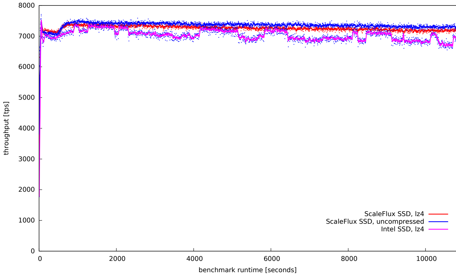
sysbench tpcc, scale 32, 32 threads, 40G BP, SSD
