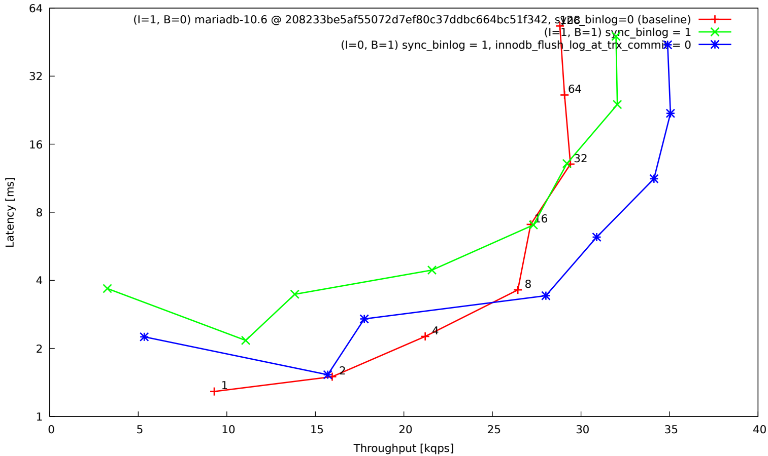
OLTP oltp_9010_read_write.lua 90:10, 16 tables, 1 mio rows each, big BP, SSD
