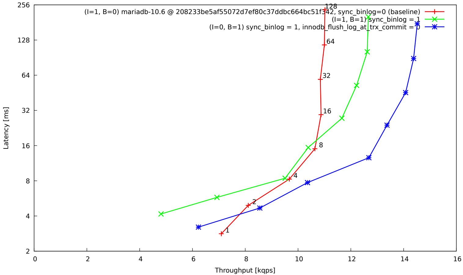
OLTP oltp_read_write.lua, 16 tables, 1 mio rows each, big BP, SSD
