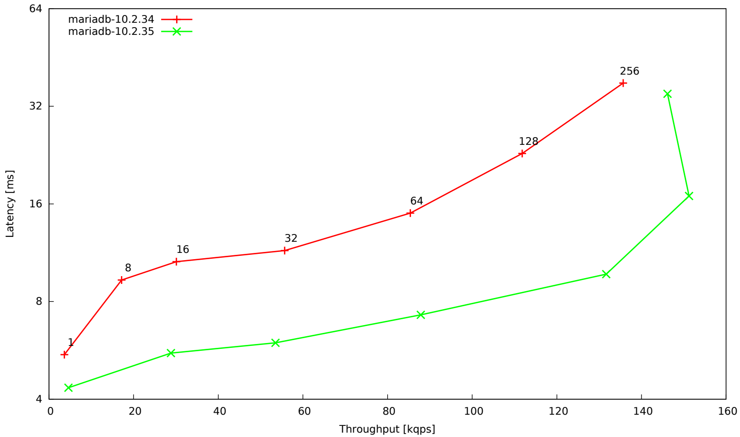
t_writes-innodb-single
