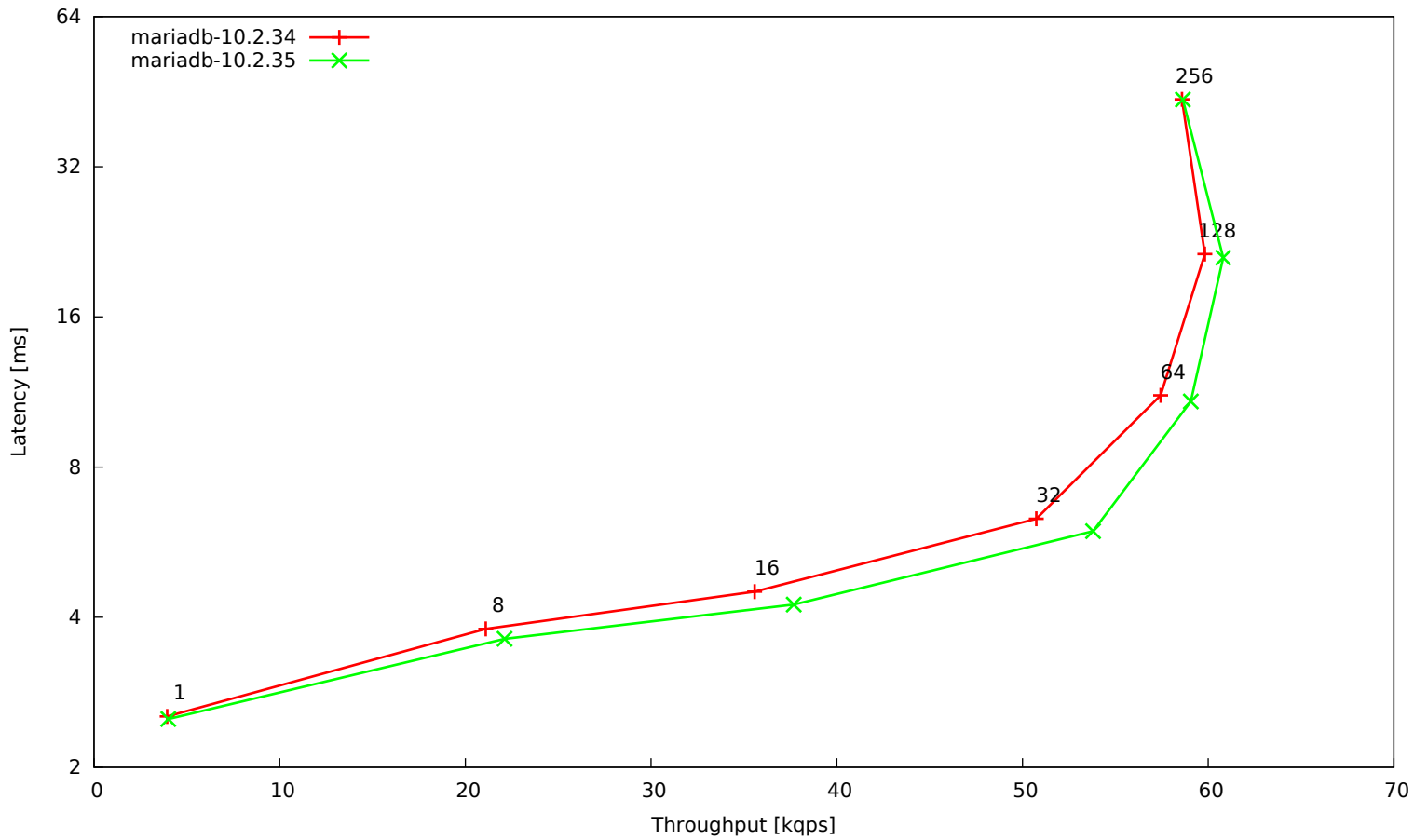
t_oltp-9010-innodb-multi
