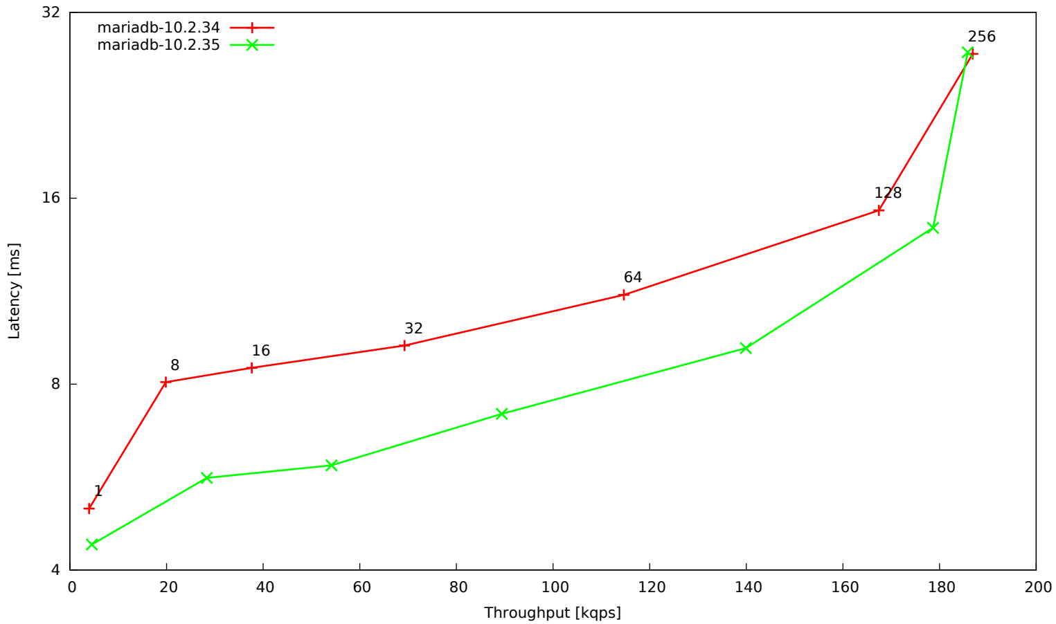
t_writes-innodb-multi
