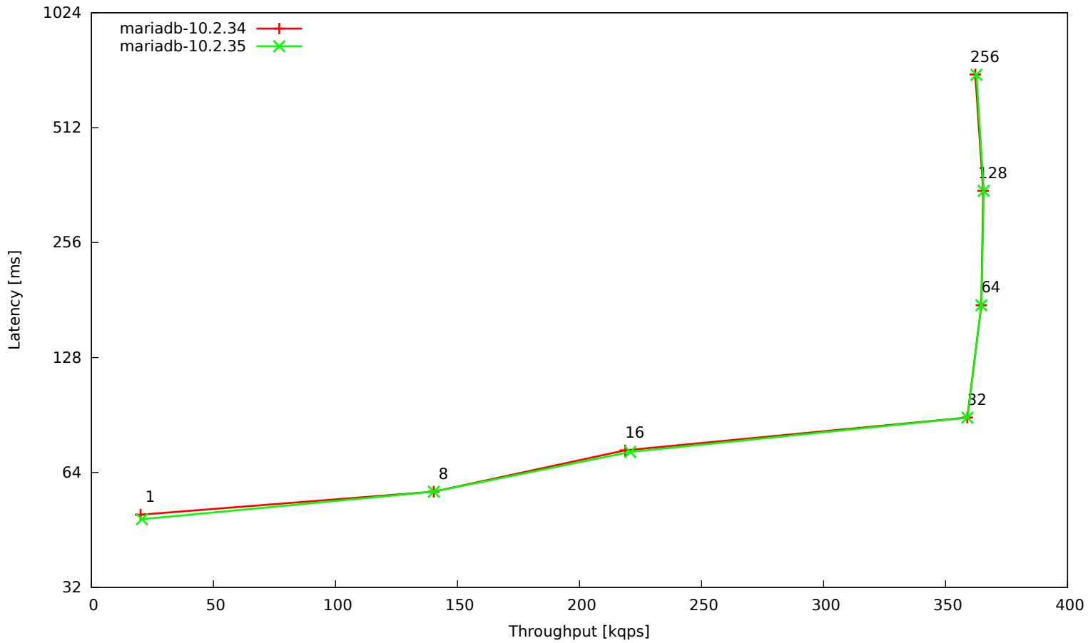
t_1K-reads-innodb-single
