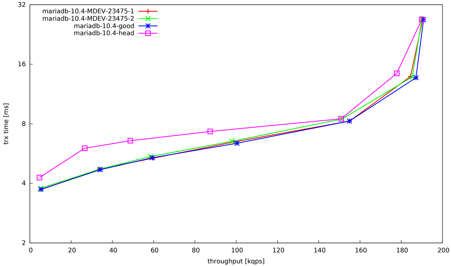
t_writes-innodb-multi
