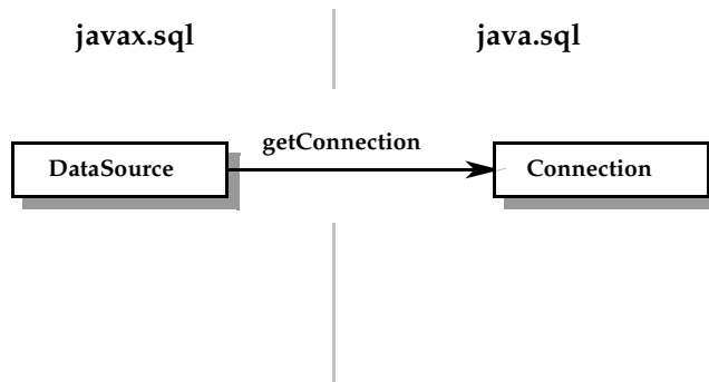
FIGURE 5-2 Relationship between javax.sql.DataSource and java.sql.Connection
